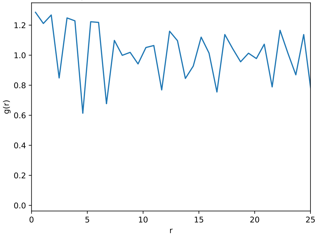
Average radial distribution function: T=0.74 , L=50
