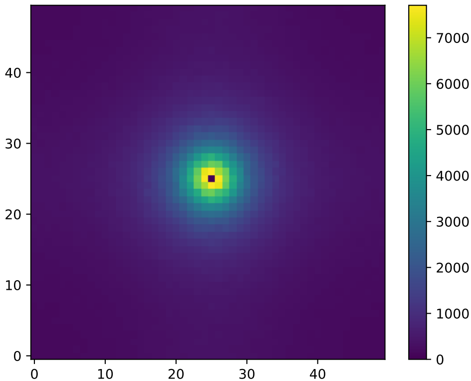
2D Structure Factor S(k) : T=0.74 , L=50
