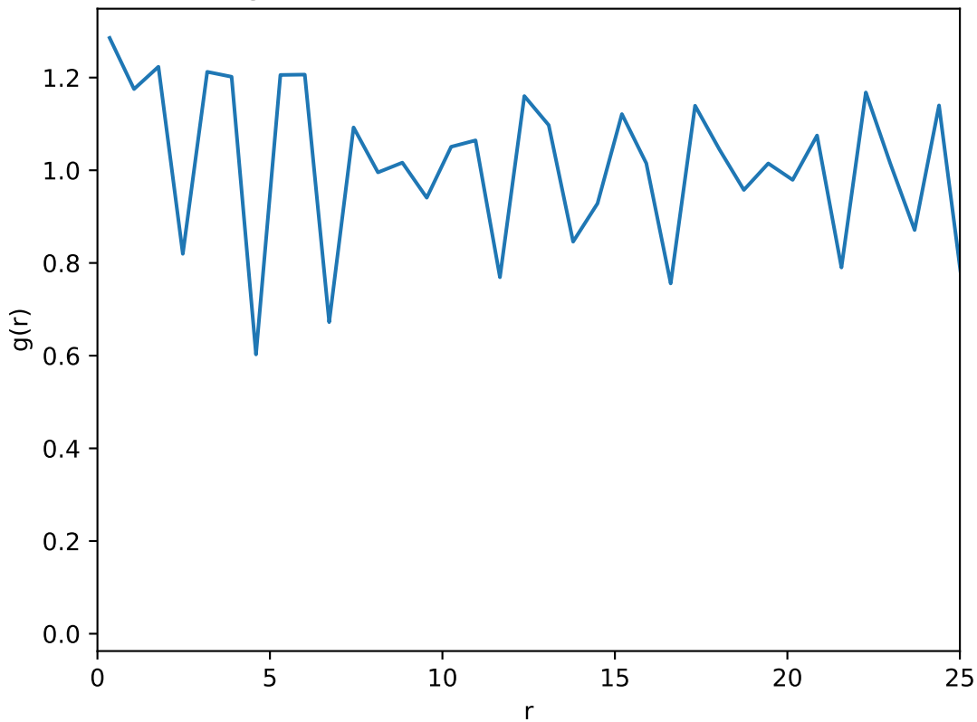
Average radial distribution function: T=0.79 , L=50
