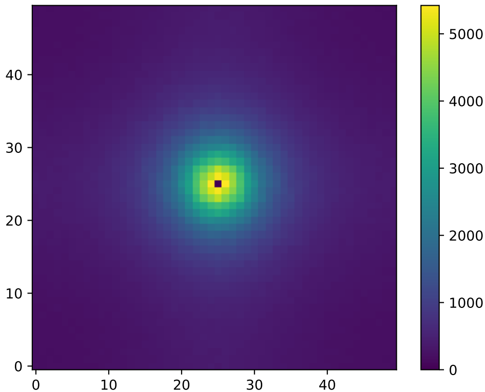
2D Structure Factor S(k) : T=0.79 , L=50
