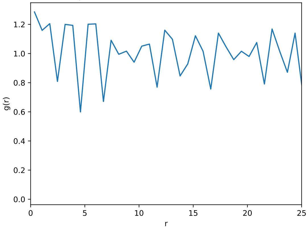
Average radial distribution function: T=0.82 , L=50
