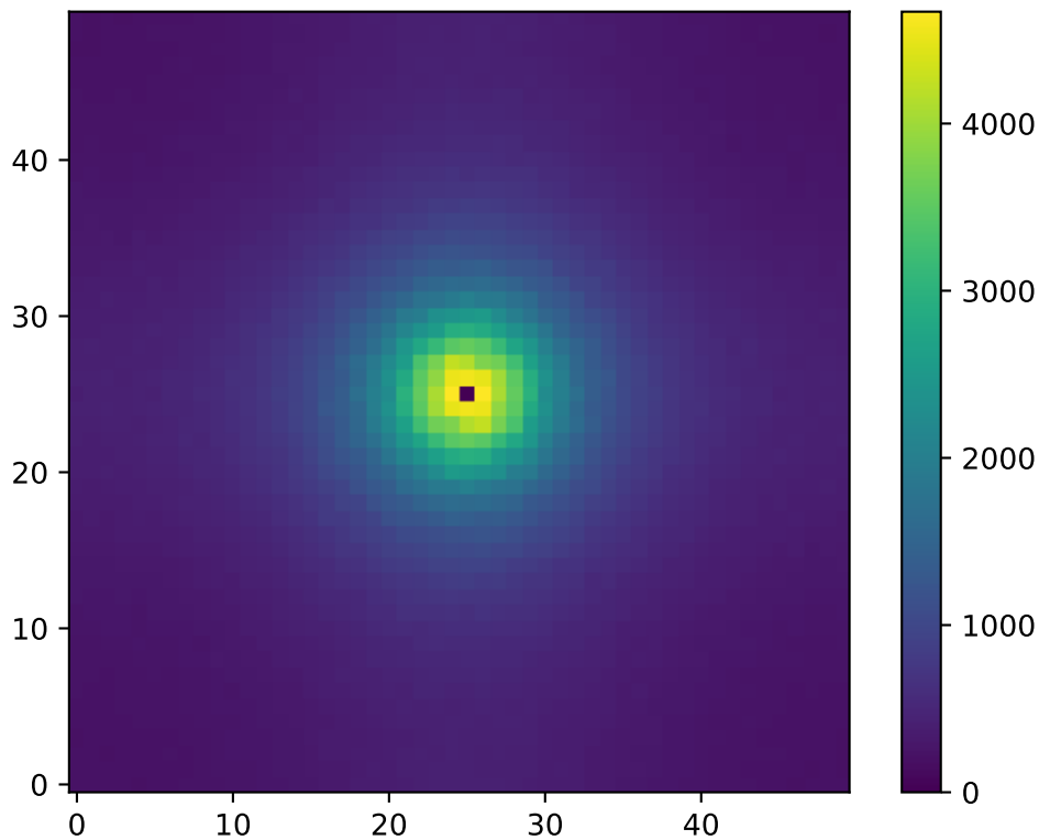
2D Structure Factor S(k) : T=0.82 , L=50
