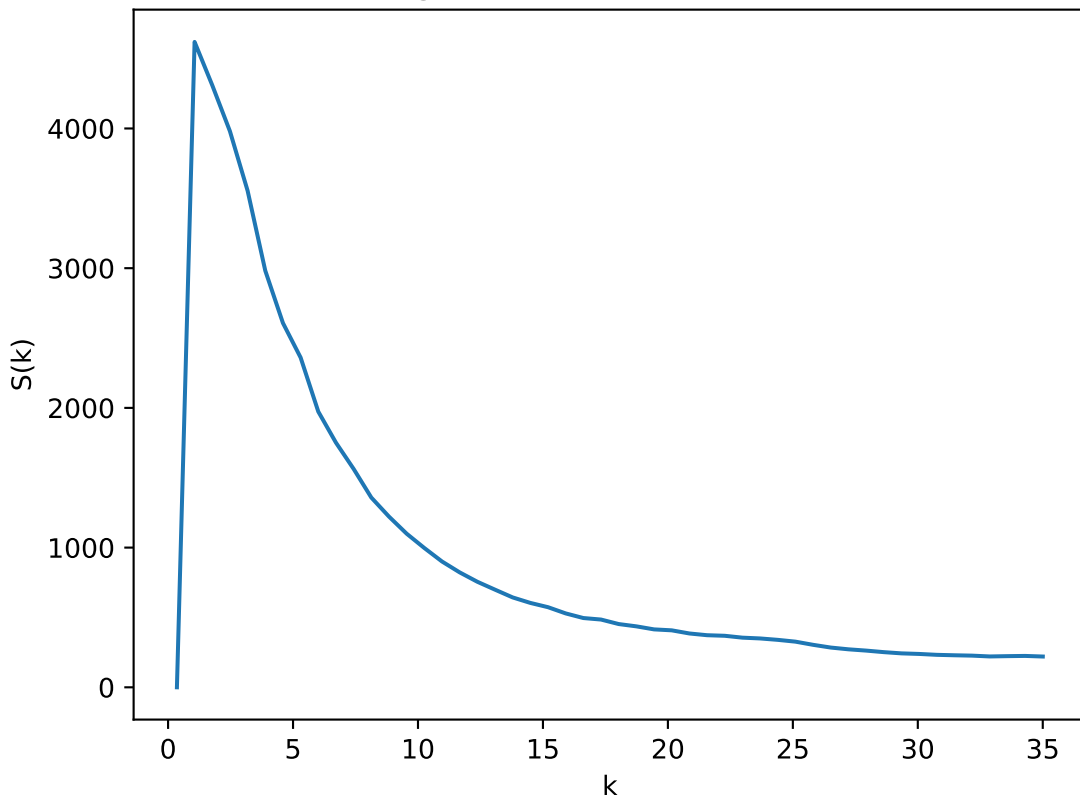
Radial Average of Structure Factor: T=0.82 , L=50
