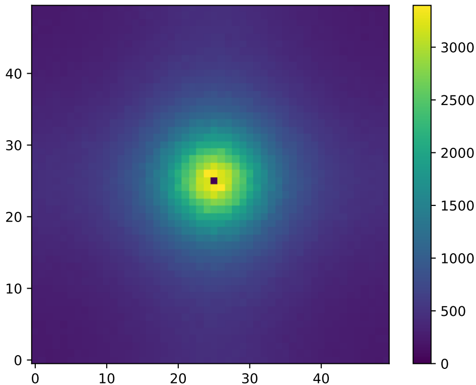
2D Structure Factor S(k) : T=0.91 , L=50
