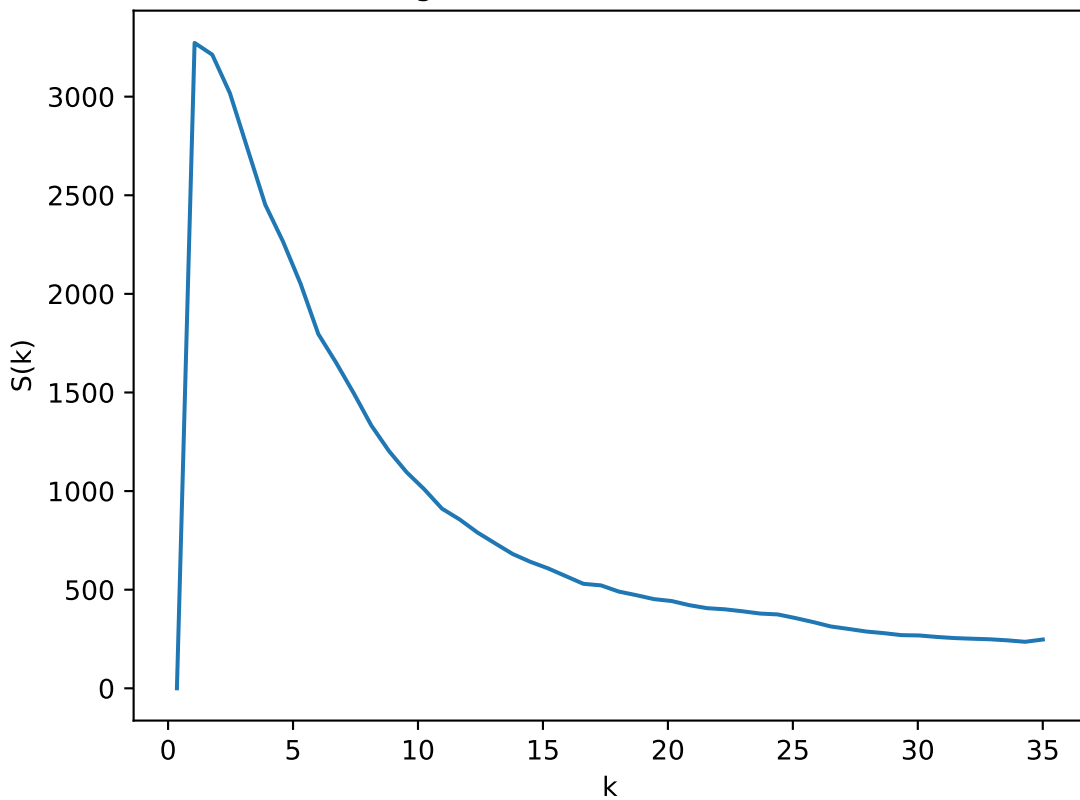
Radial Average of Structure Factor: T=0.91 , L=50
