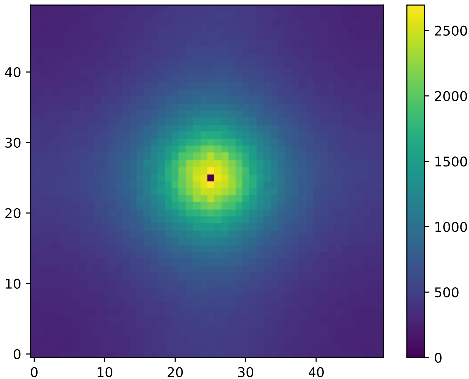
2D Structure Factor S(k) : T=1.00 , L=50
