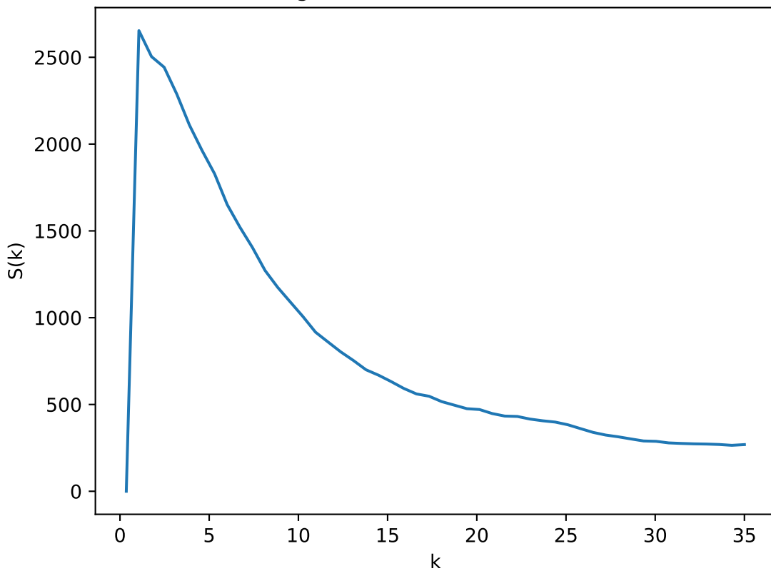
Radial Average of Structure Factor: T=1.00 , L=50
