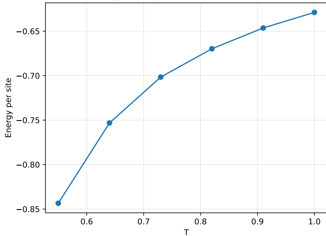
Energy vs Temperature ( L=50 , \rho=0.50 )
