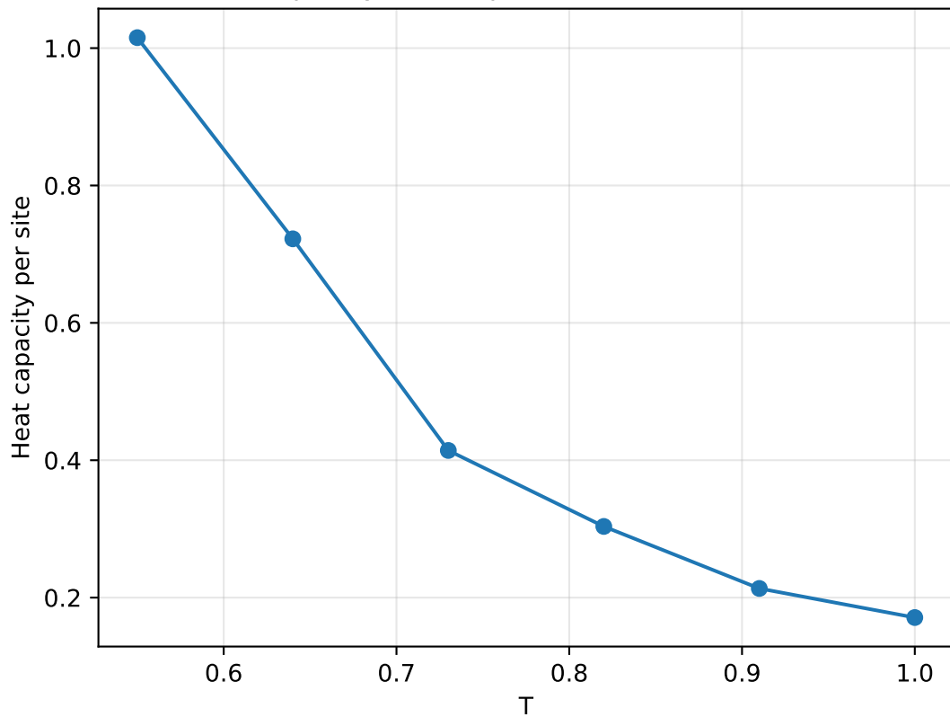
Heat Capacity vs Temperature ( L=50 , \rho=0.50 )
