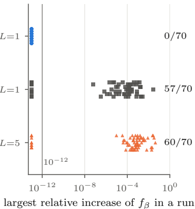
(b) 14 configurations \times 5 seeds
