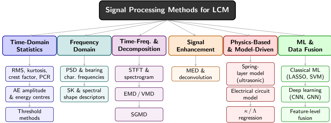
Figure 6: Taxonomy of signal processing method families applied to lubrication condition monitoring of rolling element bearings. Methods are organised by processing family rather than by sensing modality; the master cross-reference matrix (Table 4) maps each family to the sensing modalities for which LCM application has been demonstrated in the reviewed literature.
