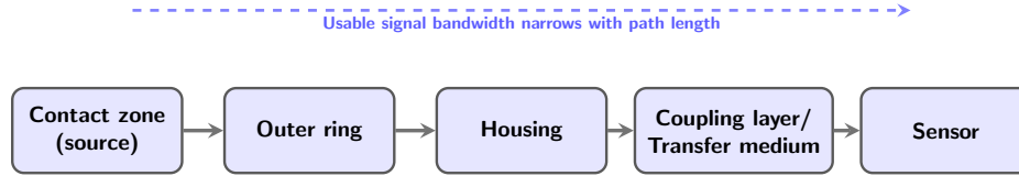
Figure 5: Signal transmission path from the ball–raceway contact zone to a housing-mounted sensor. The interface between the outer ring and housing bore – press fit, clearance fit, or clamped, depending on the bearing arrangement – is the dominant attenuation element for high-frequency content. Cumulative path losses of 30–60 dB at 500 kHz render the usable frequency bandwidth at the sensor geometry-, mounting-, and material-specific, limiting the transferability of signal processing configurations across experimental setups.
