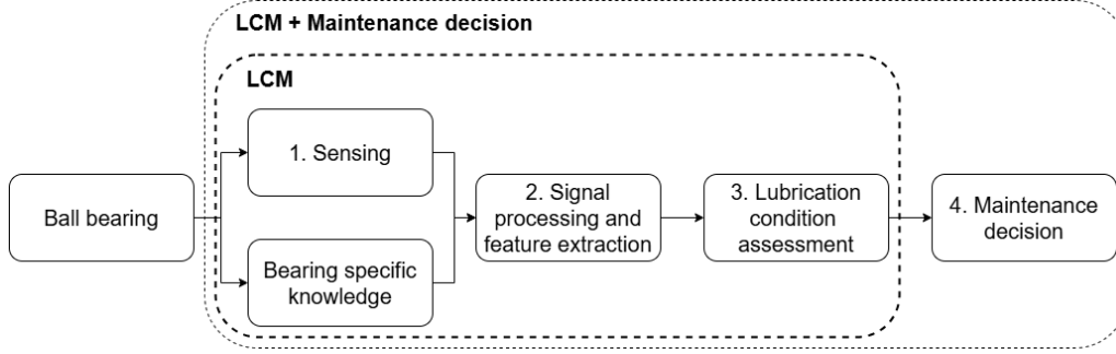
Figure 2: Steps in online LCM of a running ball bearing. Signal processing sits between the raw sensor data and the lubrication condition assessment.
