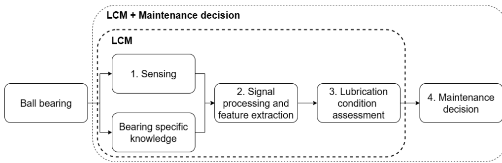
Figure 2: Steps in online LCM of a running ball bearing. Signal processing sits between the raw sensor data and the lubrication condition assessment.
