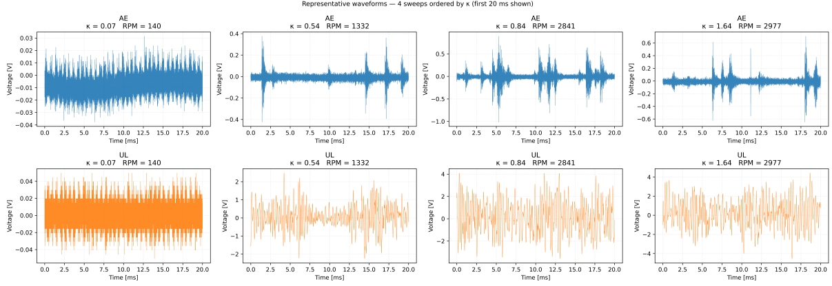
Figure 4: Waveforms of AE and US signals from the same sweeps for different values of \kappa . AE shows clear pulses of energy from asperity contacts which modulate the signal afterwards. UL shows a more regular, lower frequency, non-stationary waveform.
