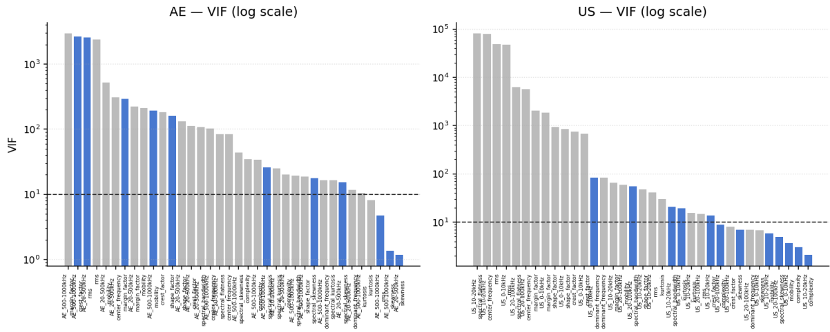
Figure 7: Variance inflation factors of the Stage 1 survivors (logarithmic axis). Retained features in blue, removed features in grey; the dashed line marks the VIF = 10 qualifier used by the Stage 2 pairwise removal. Values are capped at 10^6 for display.
