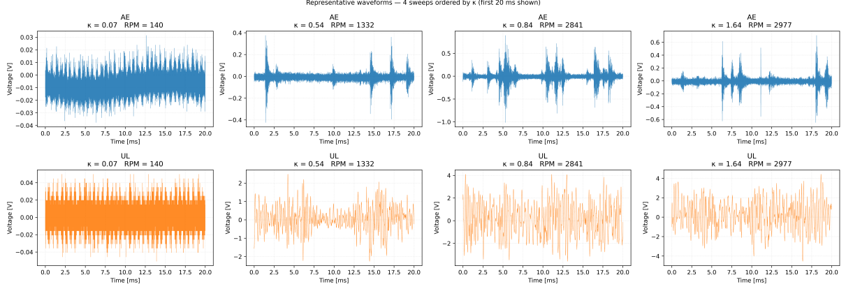
Figure 4: Waveforms of AE and US signals from the same sweeps for different values of \kappa . AE shows clear pulses of energy from asperity contacts which modulate the signal afterwards. US shows a more regular, lower frequency, non-stationary waveform.
