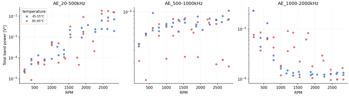
Figure 5: Total AE band power as a function of RPM at two fixed temperature windows. The 20–500 kHz band rises monotonically with speed; the 1–2 MHz band decays to a common electronics floor at a temperature-dependent speed, i.e. at a comparable lubrication state ( \kappa ) rather than a comparable RPM.
