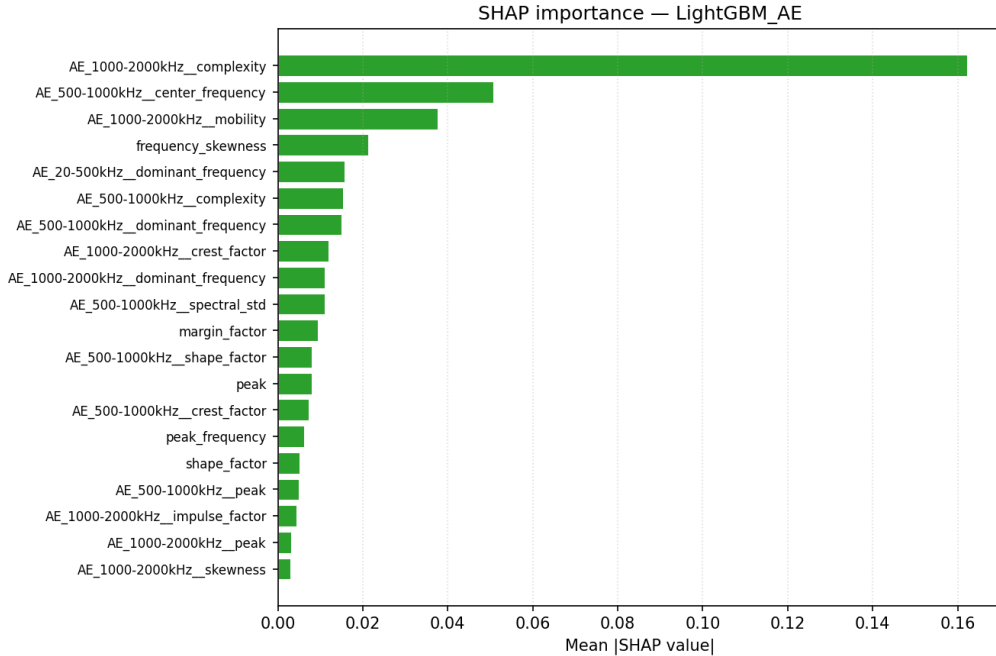
Figure 11: SHAP feature importance (mean |\text{SHAP value}| ) for the LightGBM model trained on AE features. Features from frequency sub-bands are prefixed with the band label (e.g., AE_20–500kHz_).
