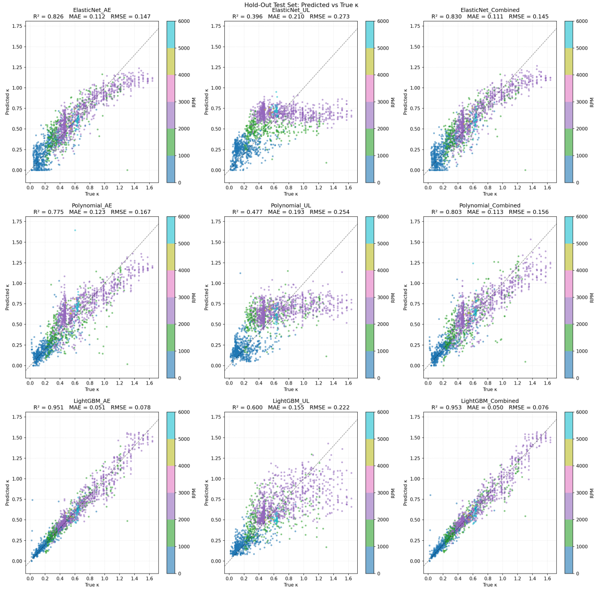
Figure 10: Predicted vs. actual \kappa on the hold-out test set for all model families and sensor configurations, colored according to RPM. The dashed diagonal indicates perfect prediction. Residual spread increases in the mixed lubrication regime ( 0.5 \leq \kappa < 1.0 ).
