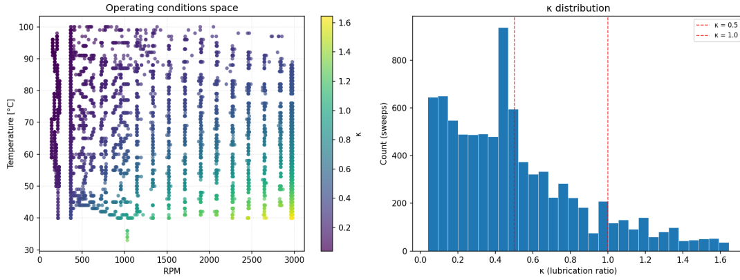
Figure 2: Left: space of the measured operating conditions (RPM and temperature) during the experiment. Each point corresponds to a 20ms window of sampling at a given RPM and temperature. The colour of each point corresponds to the derived \kappa value for that sweep, with warmer colours indicating higher \kappa values. Right: distribution fo the derived \kappa values.
