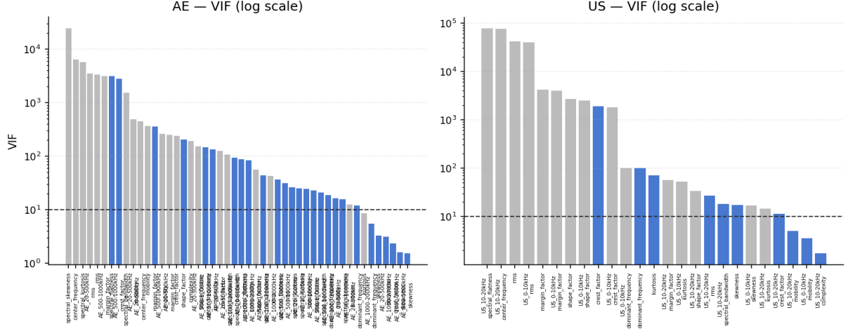
Figure 6: Variance inflation factors of the Stage 1 survivors (logarithmic axis). Retained features in blue, removed features in grey; the dashed line marks the VIF = 10 qualifier used by the Stage 2 pairwise removal. Values are capped at 10^6 for display.
