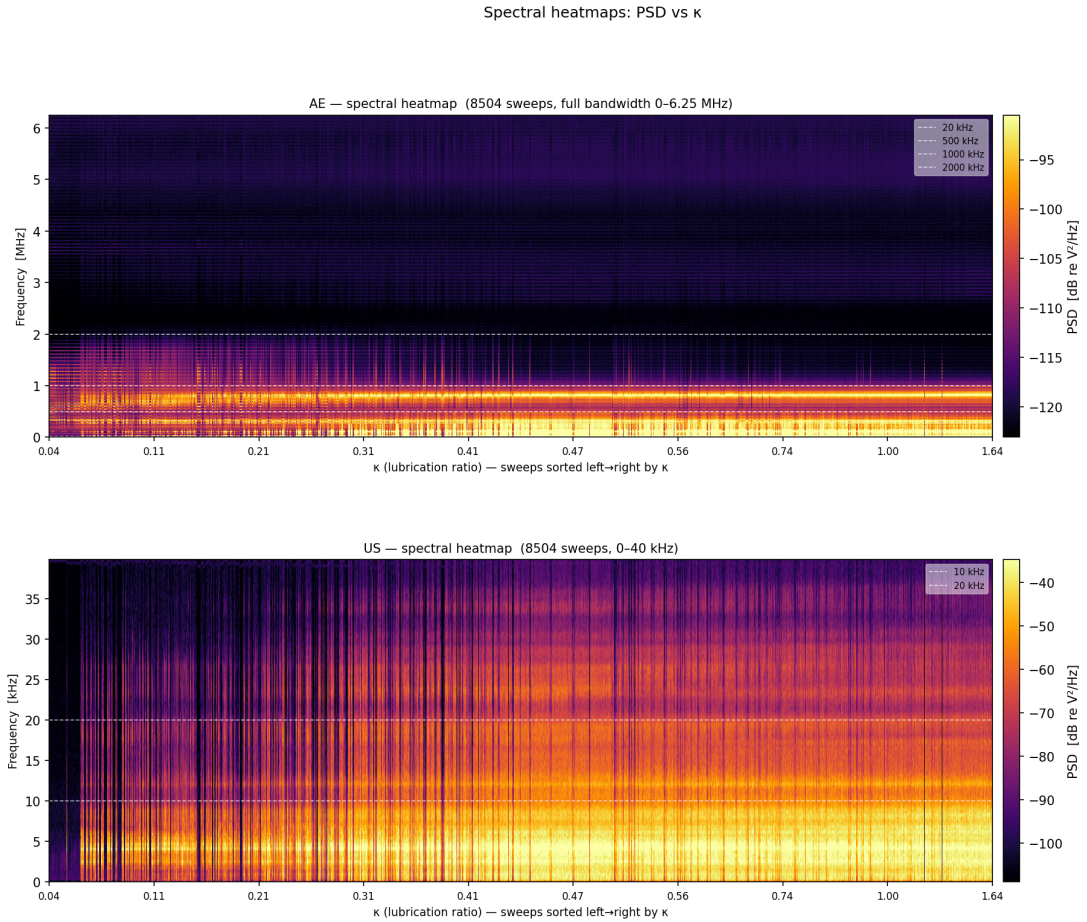
Figure 4: Spectrograms of the raw AE and US signals across the operating conditions. Each column corresponds to a sweep, sorted by increasing \kappa value from left to right. The colour indicates the magnitude of the signal in dB, with warmer colours indicating higher magnitudes.
