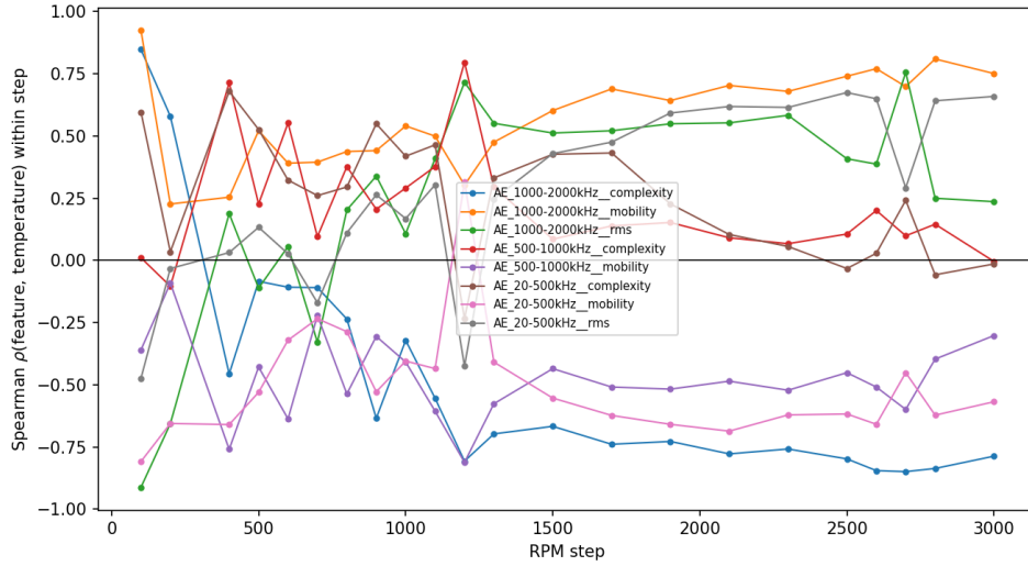
Figure 7: Within-RPM-step Spearman correlation between selected AE sub-band features and temperature. At fixed speed the drive state is constant, so non-zero correlations reflect sensitivity to the lubrication state rather than to the operating point.
