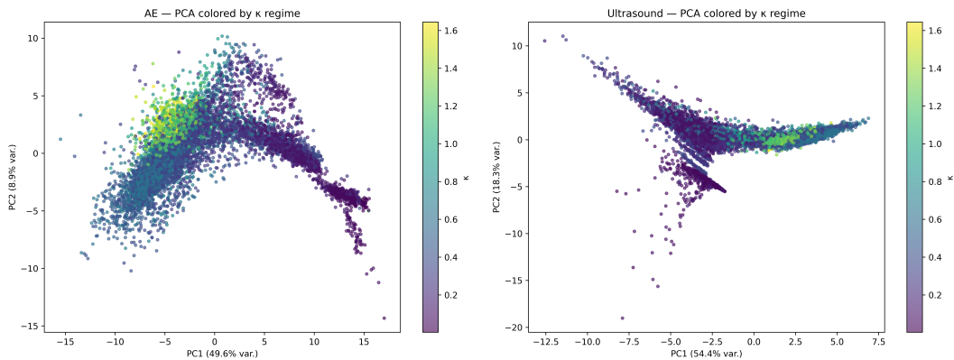
Figure 8: PCA projection of the retained AE and US feature sets, coloured by lubrication \kappa value.
