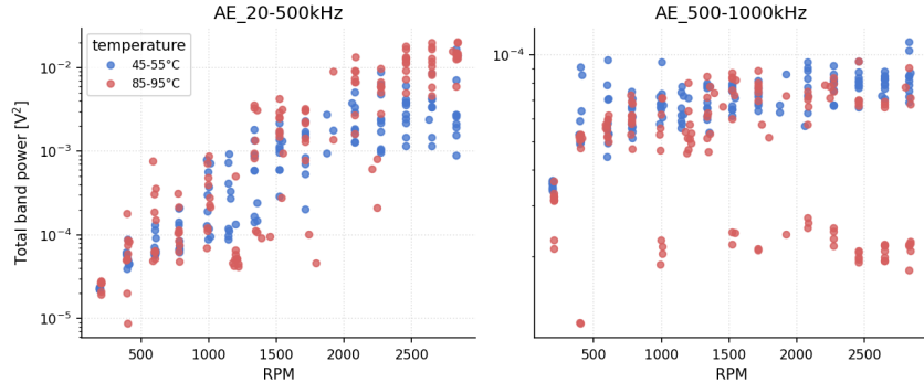
Figure 6: Total power of the two retained AE sub-bands as a function of RPM at fixed temperature windows. Both bands rise with speed, consistent with mechanically generated emission.
