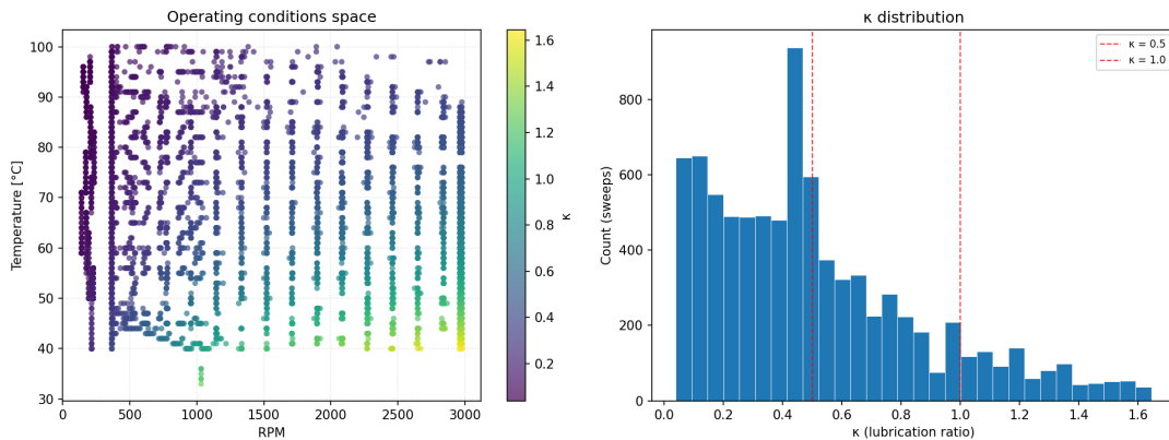
Figure 1: Left: space of the measured operating conditions (RPM and temperature) during the experiment. Each point corresponds to a 20ms window of sampling at a given RPM and temperature. The colour of each point corresponds to the derived \kappa value for that sweep, with warmer colours indicating higher \kappa values. Right: distribution of the derived \kappa values.
