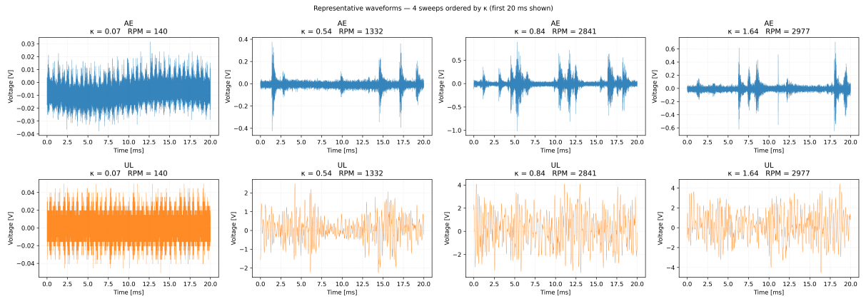
Figure 3: Waveforms of AE and UL signals from the same sweeps for different values of \kappa . AE shows clear pulses of energy from asperity contacts which modulate the signal afterwards. UL shows a more regular, lower frequency, non-stationary waveform.
