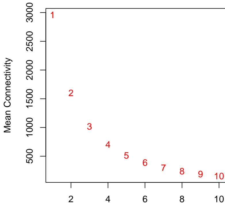
Mean connectivity
