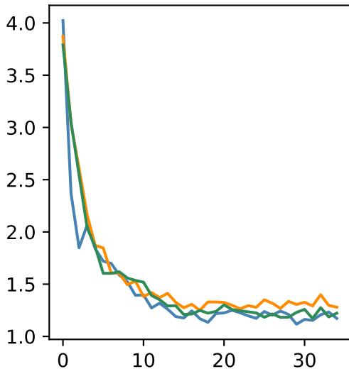
Average Loss
