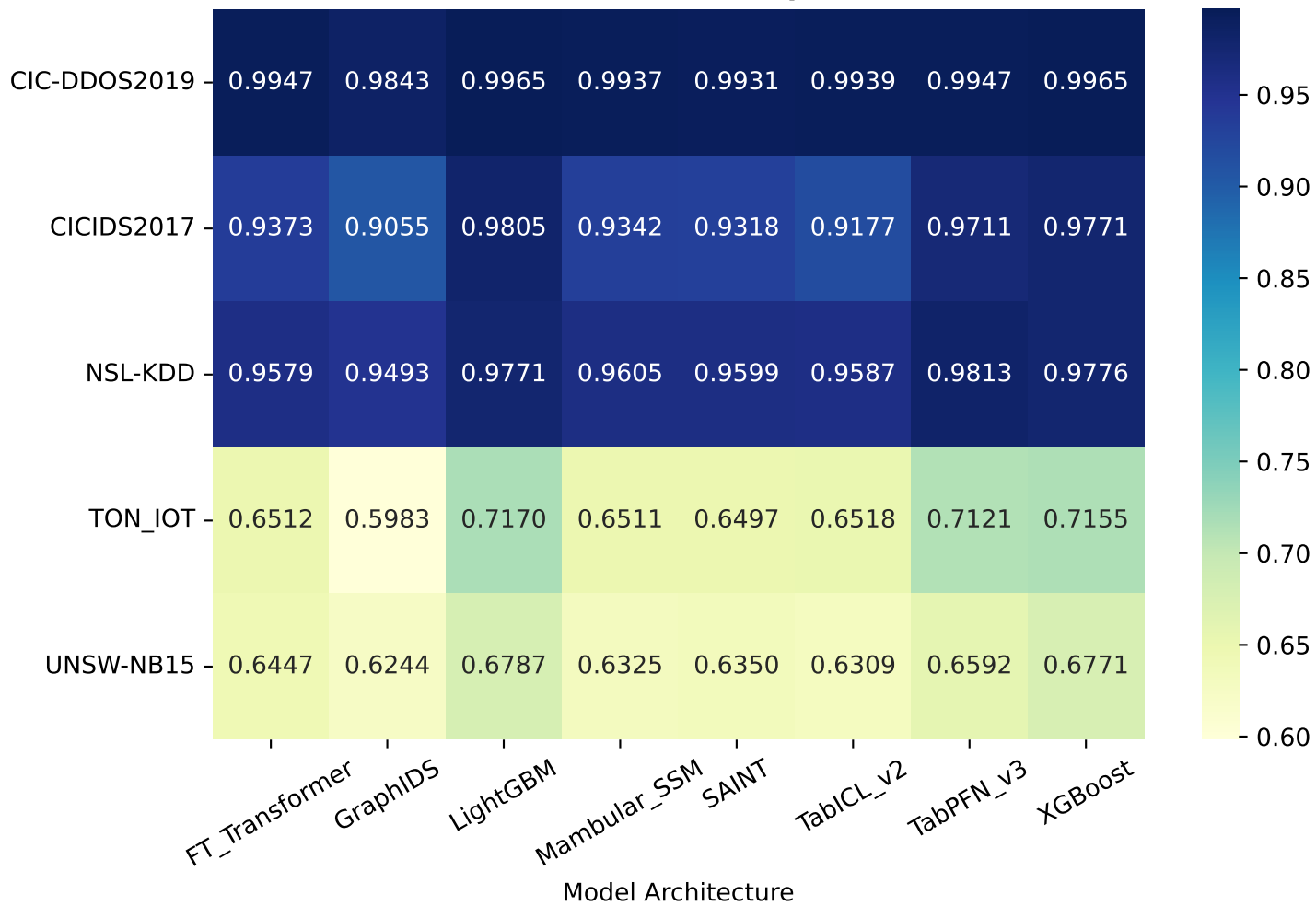
C. Cross-Dataset Generalization Heatmap (5 Datasets × 8 Models)
