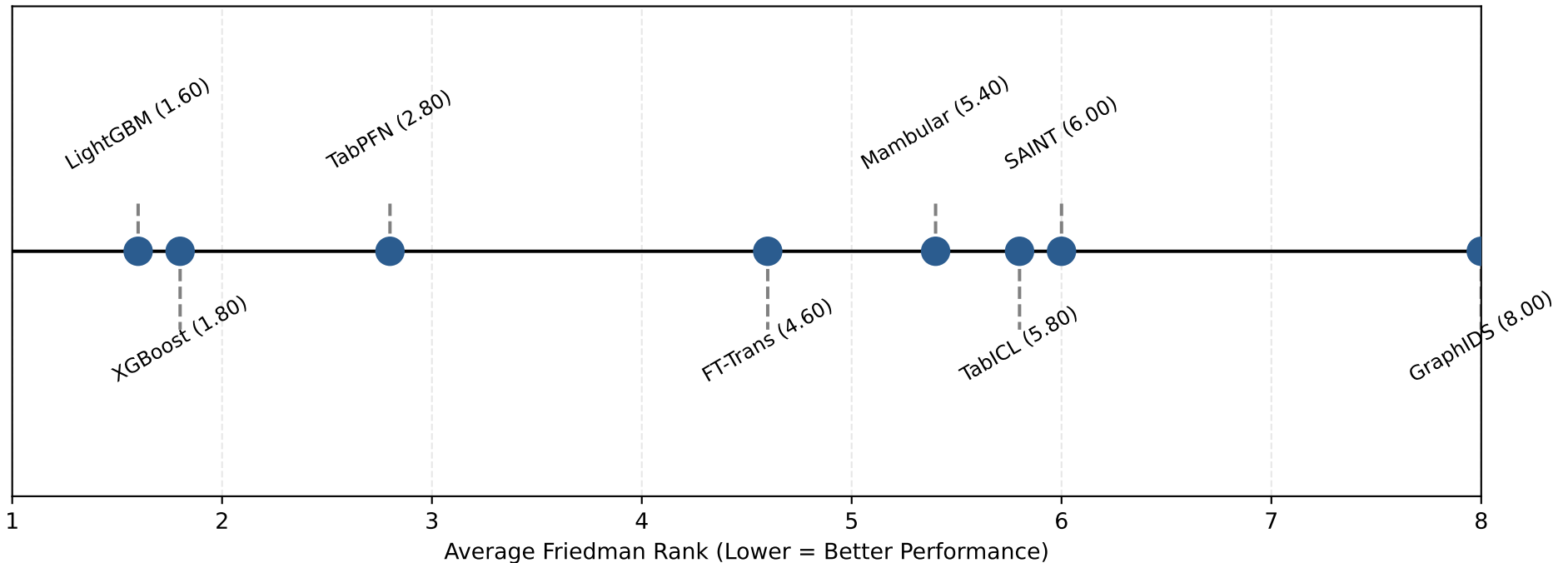
Critical Difference Diagram (Nemenyi CD = 4.696, \alpha=0.05 )
