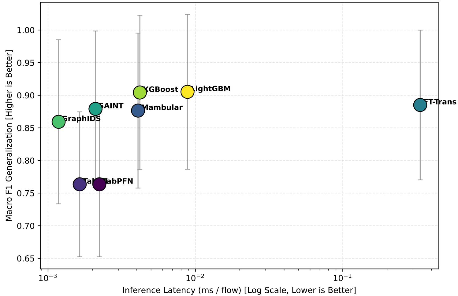
Publication Figure: TTF Accuracy vs. Per-Flow Latency Frontier (REAL MULTI-DATASET (5 Datasets))
