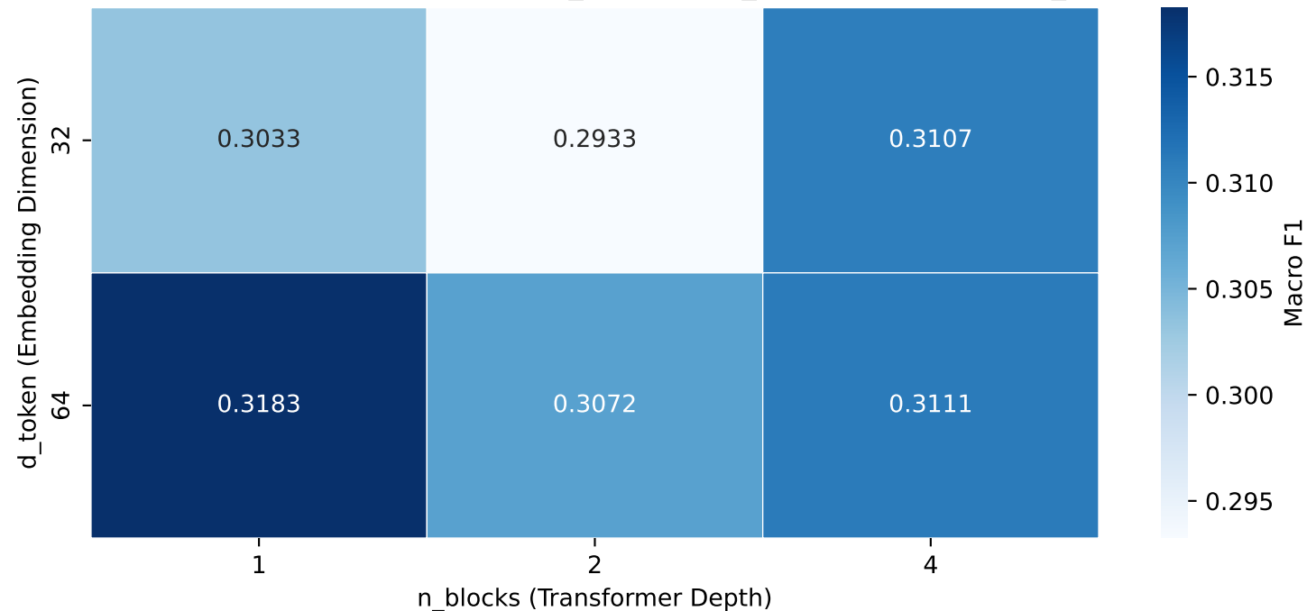
FT-Transformer Parametric Ablation: d_token vs. n_blocks (mean over n_heads)
