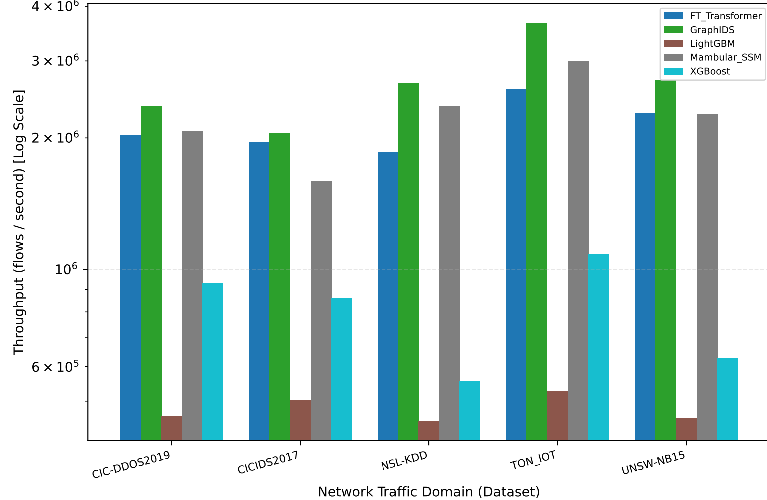
D. Cross-Domain Throughput Robustness (N=100,000 flows)
