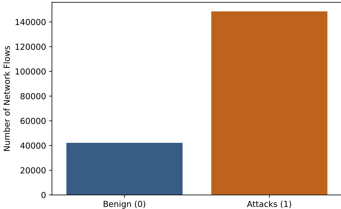
Class Distribution: TON_IOT (Decontaminated)
