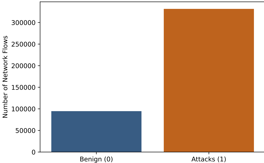
Class Distribution: CIC-DDOS2019 (Decontaminated)
