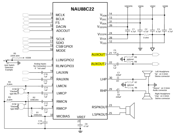
11.1 Typical Application Schematic
