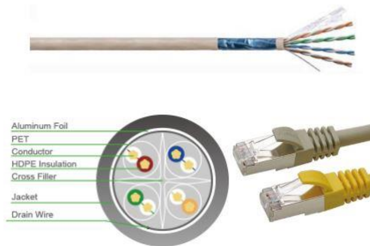
Vivanco Copper Patch Cord Cat-6 F/UTP
