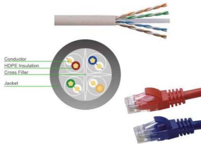
Vivanco Copper Patch Cord Cat-6 U/UTP
