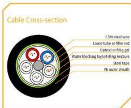
Vivanco Fiber Optic Armored Cable Multi Mode with Steel Tape & PE Sheath
