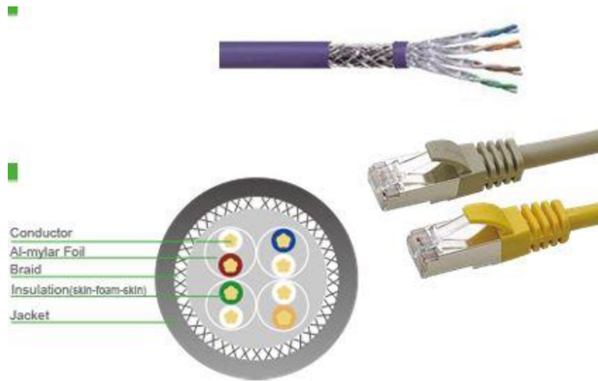
Vivanco Copper Patch Cord Cat-6A S/FTP
