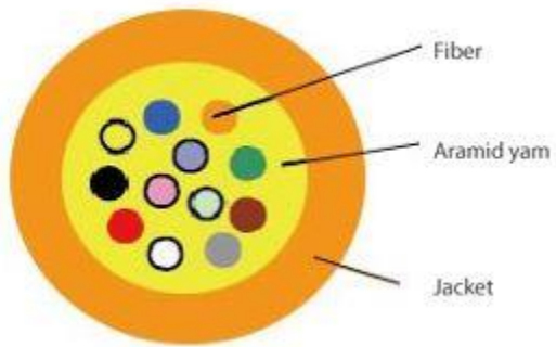
Vivanco Indoor Tight Buffer Optical Fiber Cable Single Mode
