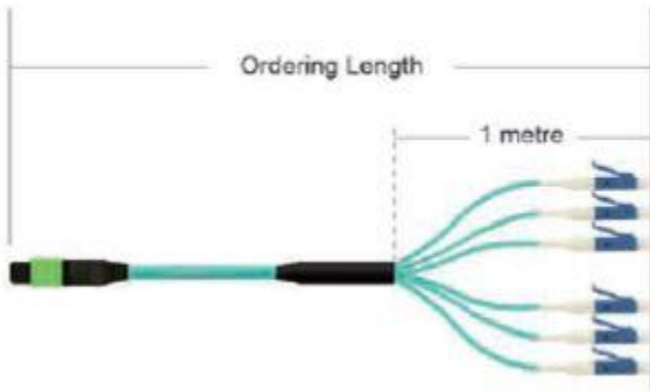
Vivanco Fiber Patch Cord MTO
