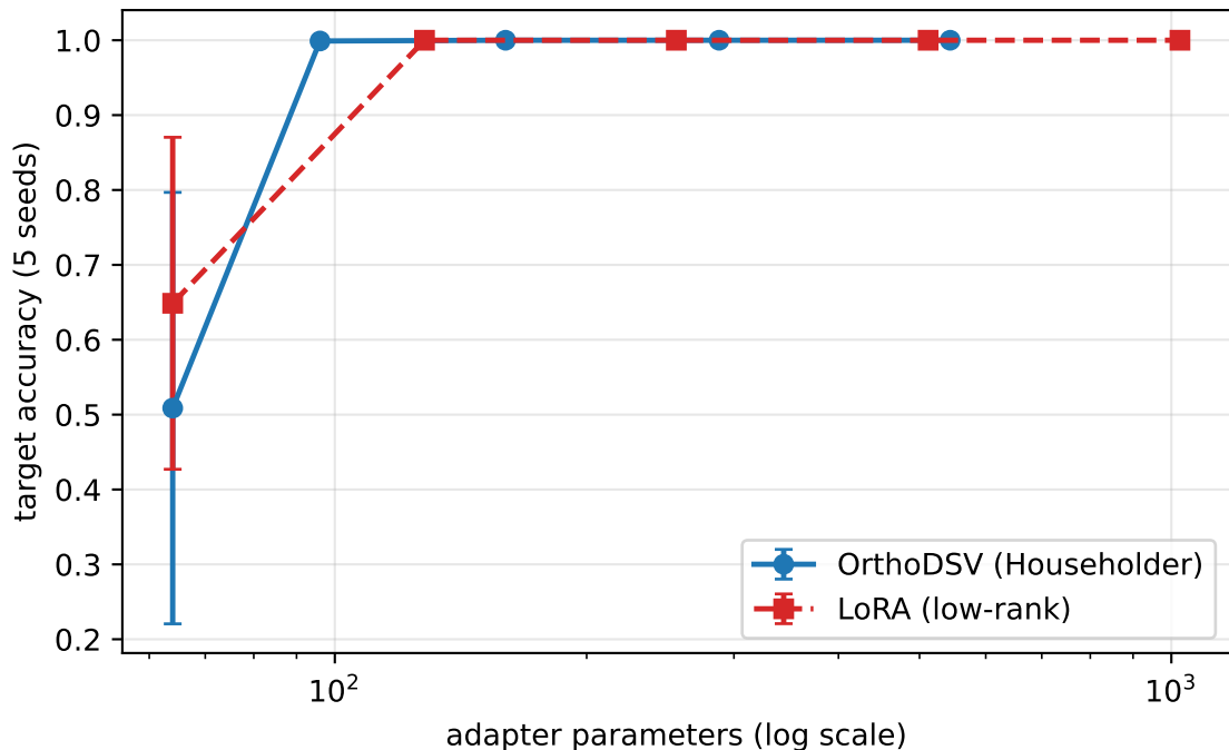
Stage-1 Pareto: orthogonal alignment vs low-rank (rotation + translation shift)
