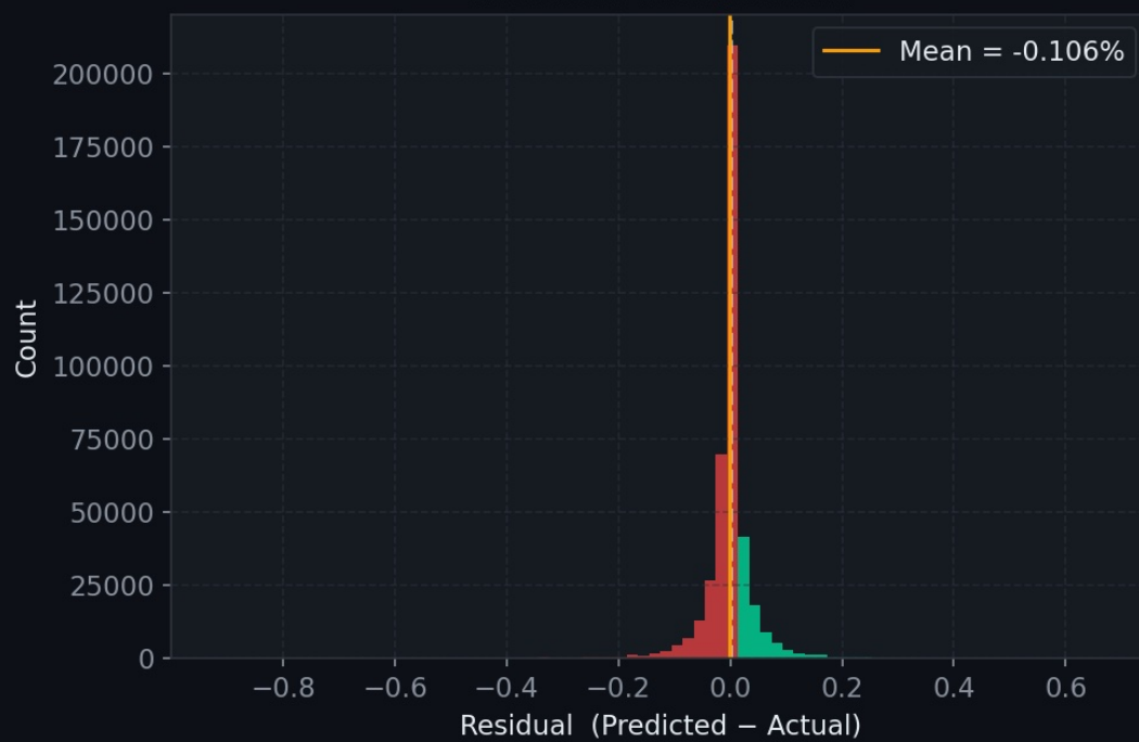
Residual Distribution
