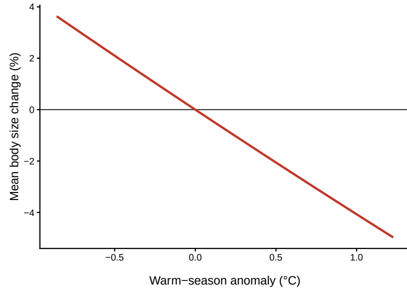
d Fished taxa lose most per degree of warming
