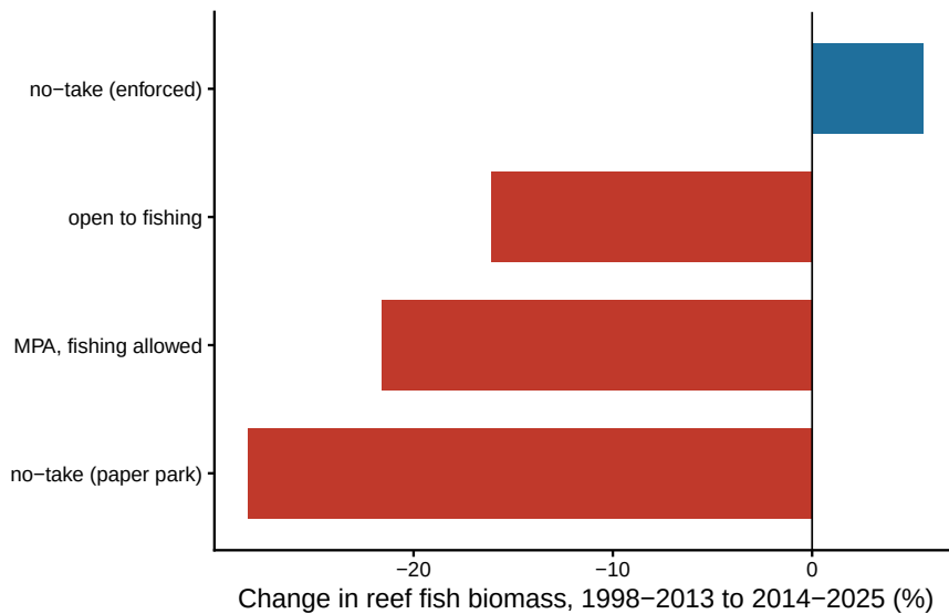
c Only enforced no-take held its biomass
