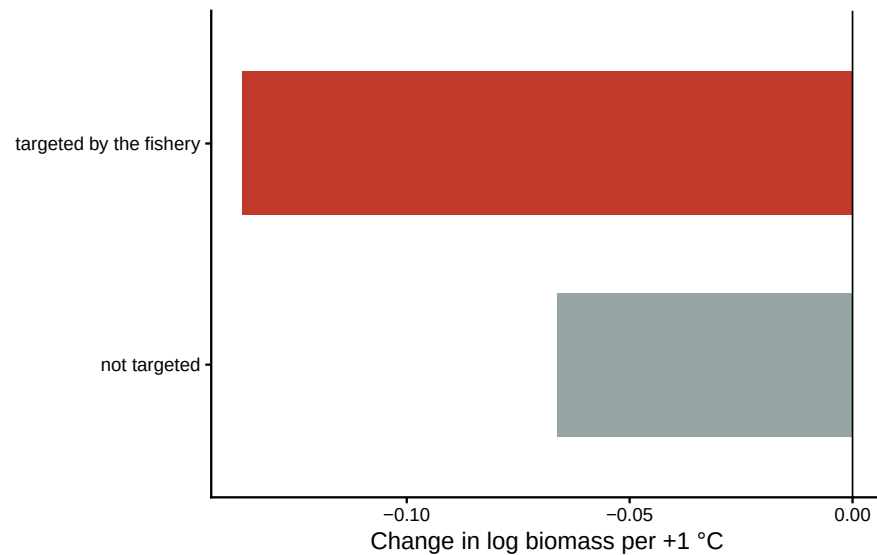
d Fished taxa lose most per degree of warming
