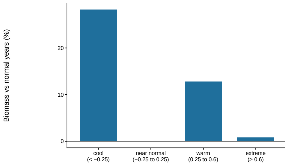
a Reef fish tolerate warm years until about +0.6 °C
