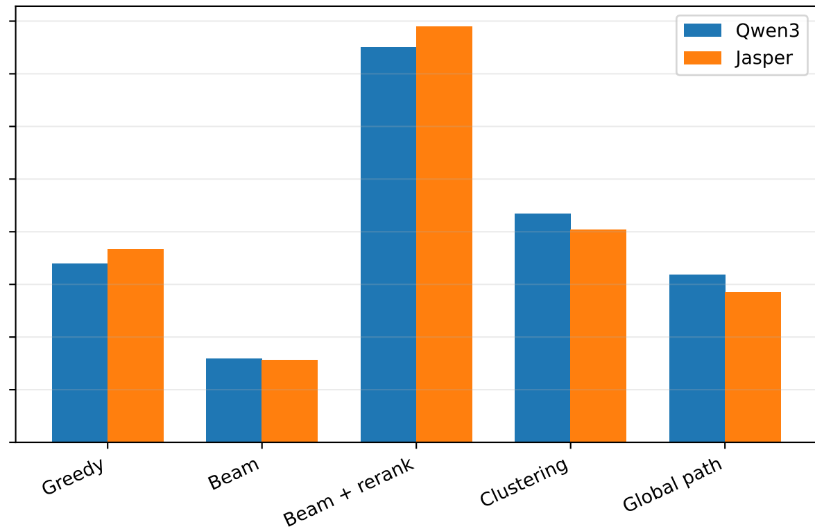
Cross-encoder
