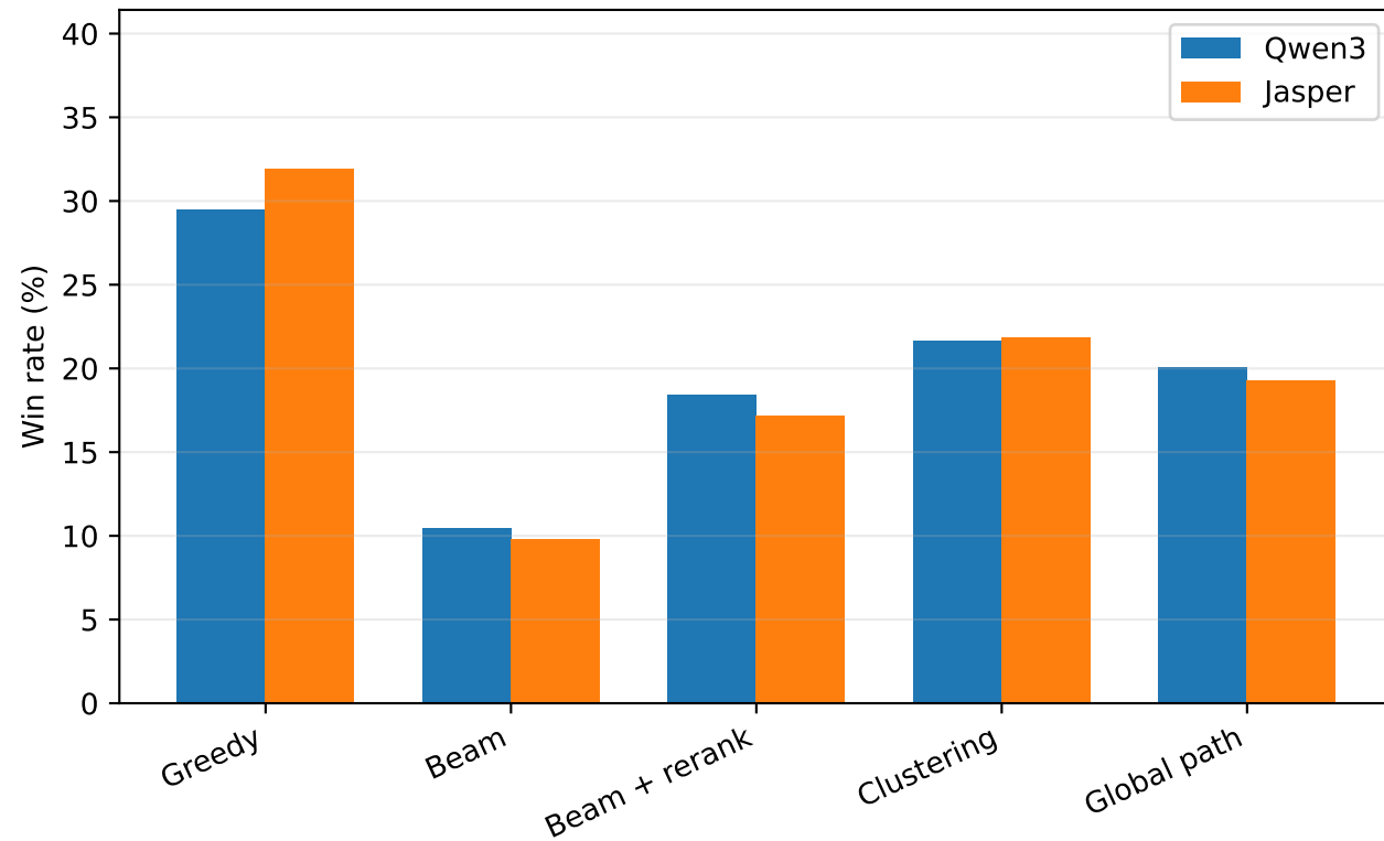
Bi-encoder
