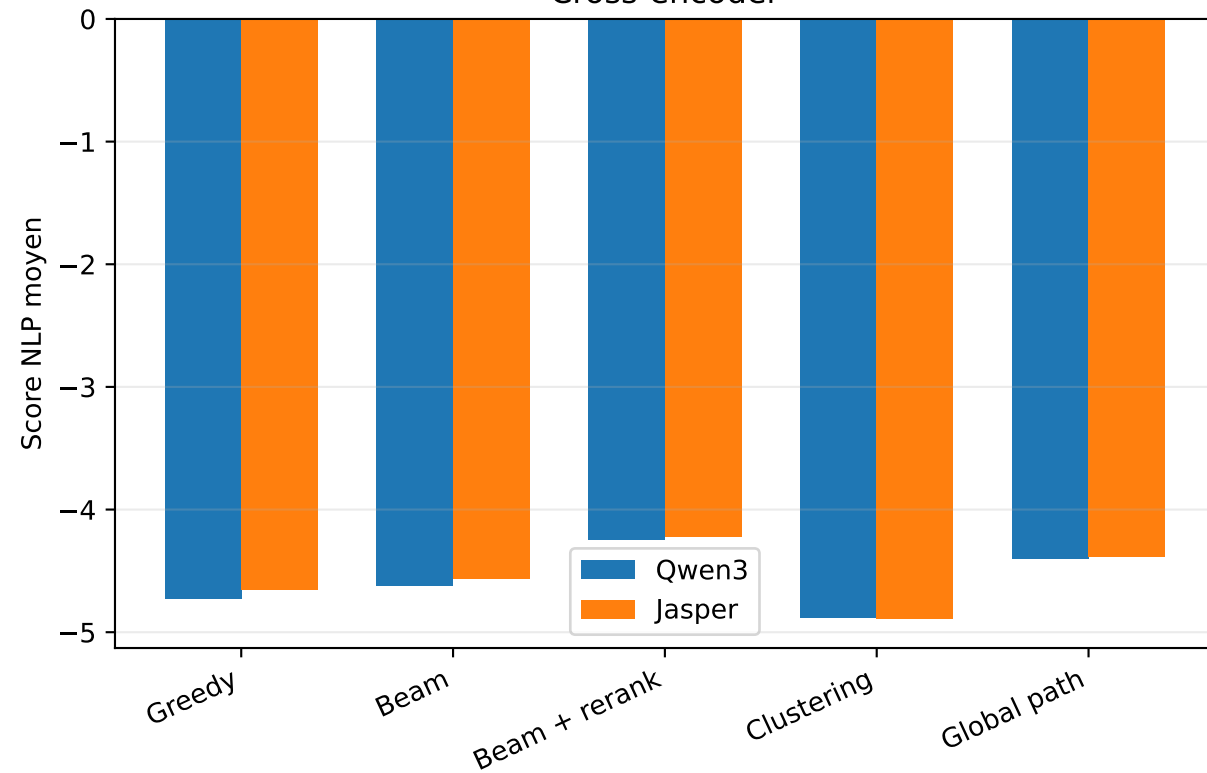
Cross-encoder
