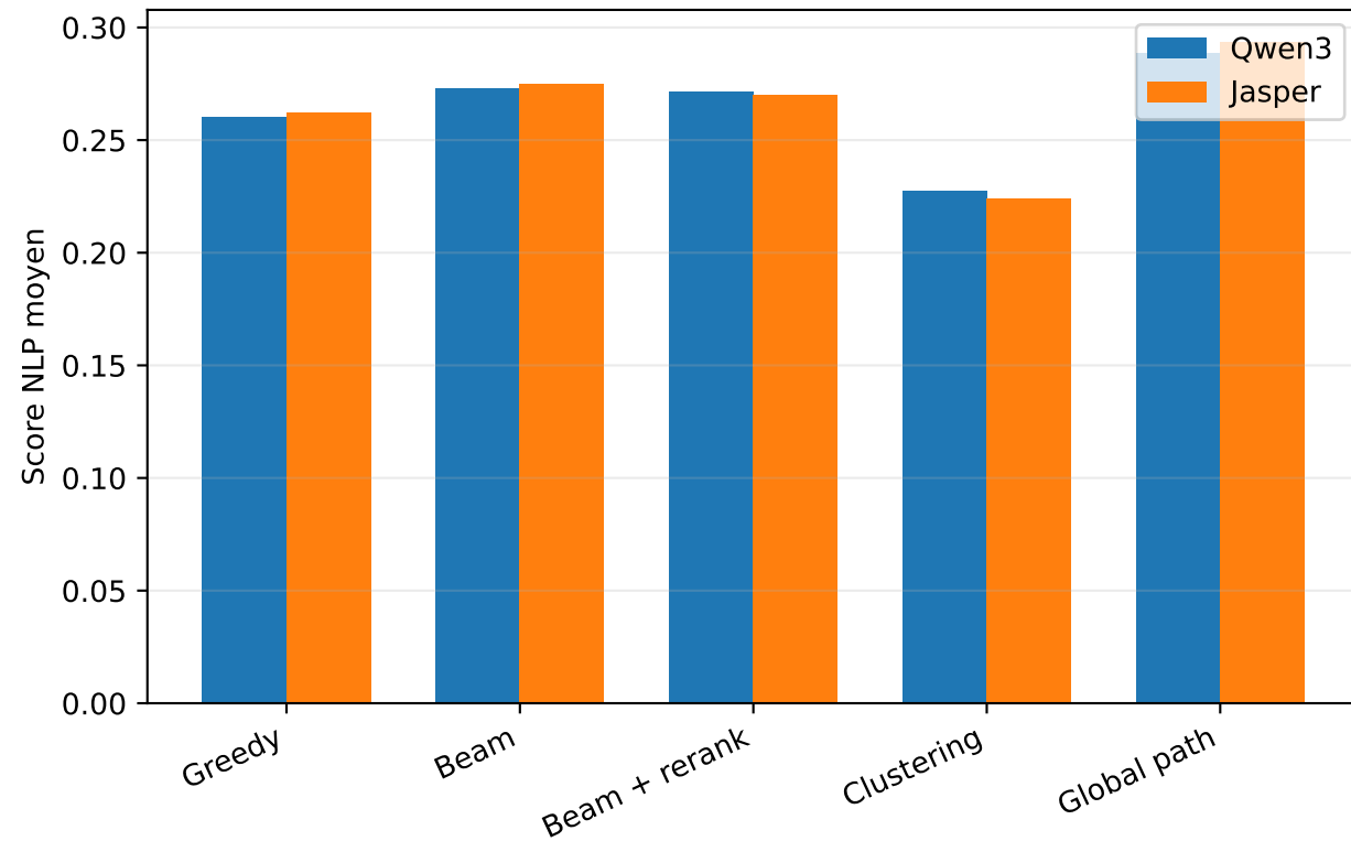
Bi-encoder
