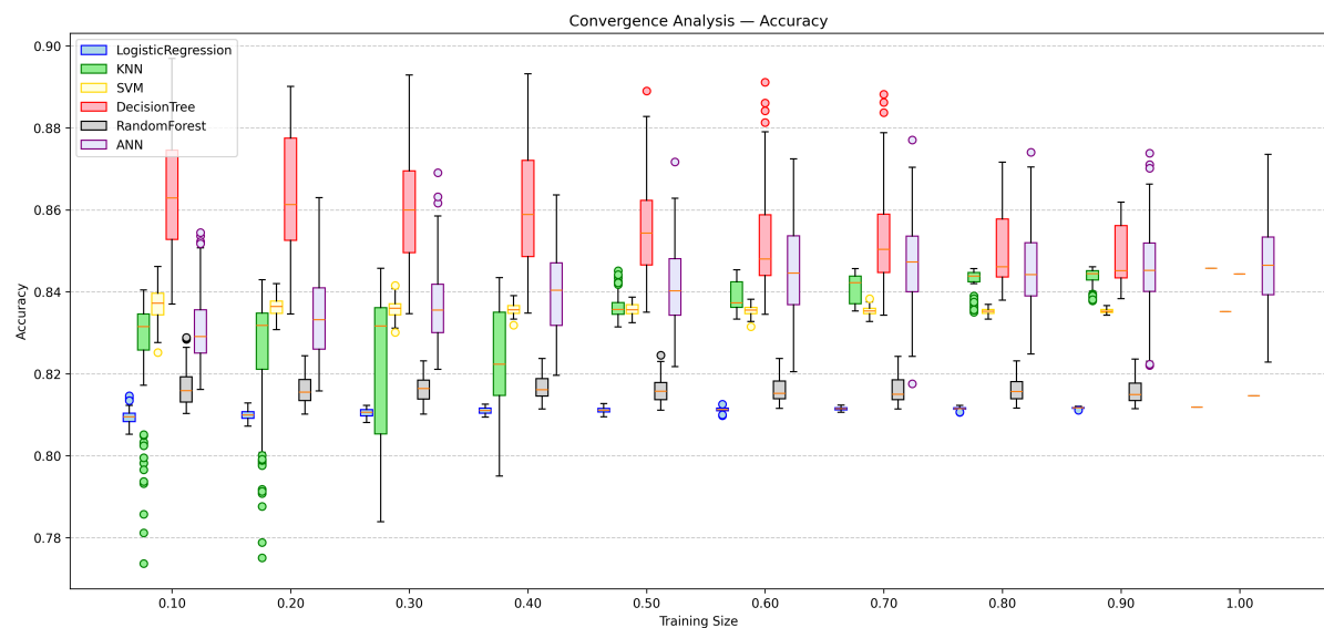
Figure 7: Convergence box plots, Accuracy, Dataset 2.
