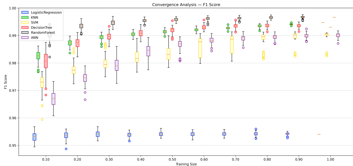
Figure 6: Convergence box plots, Weighted F1, Dataset 1.
