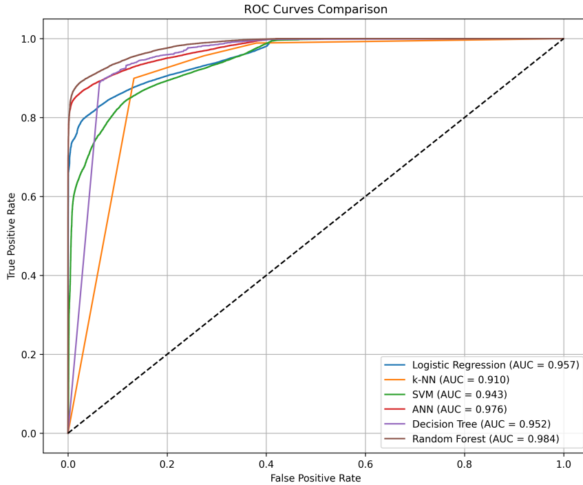
Figure 4: ROC curves for all six models on Dataset 2.
