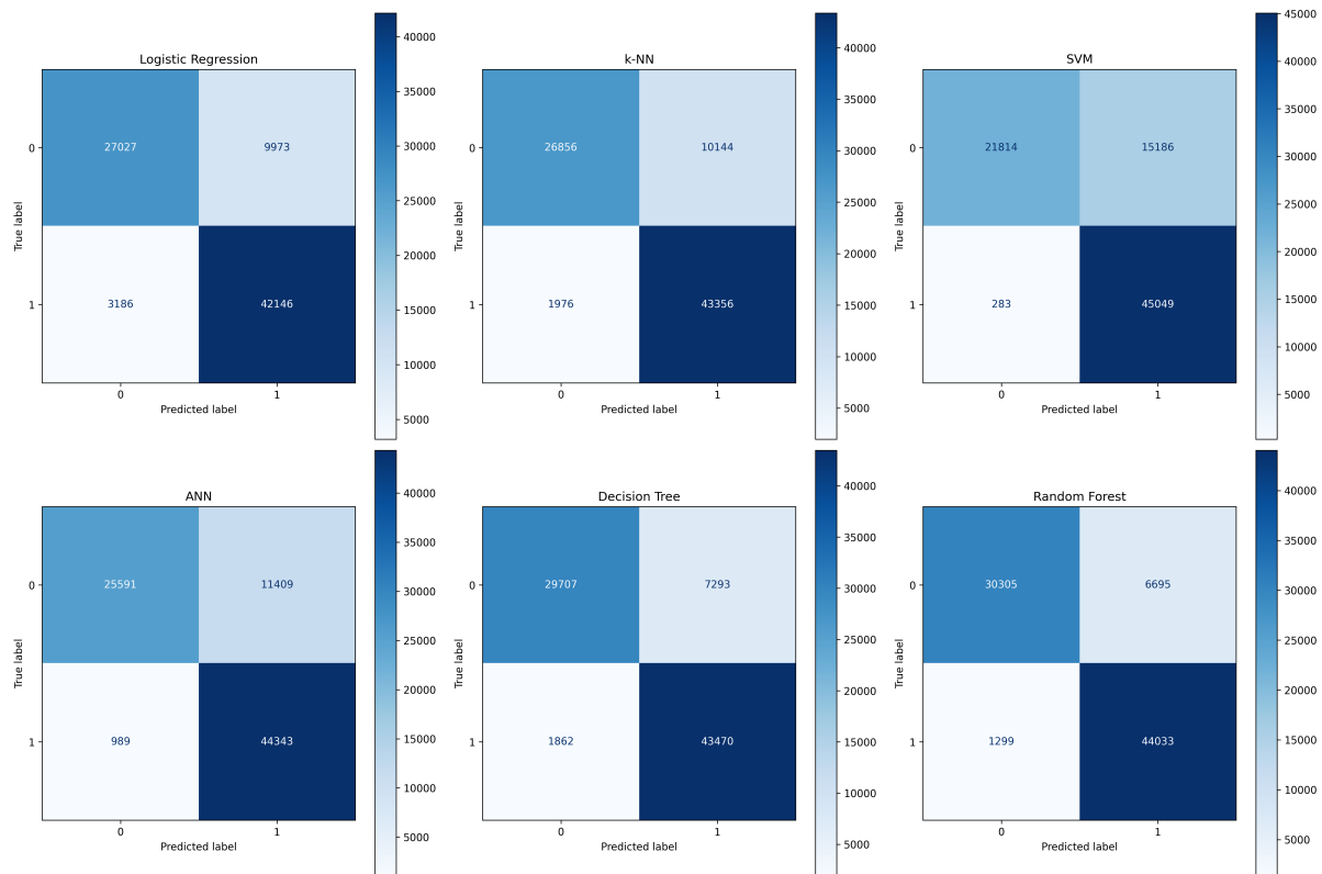
Figure 2: Confusion matrices for all six models on Dataset 2.
