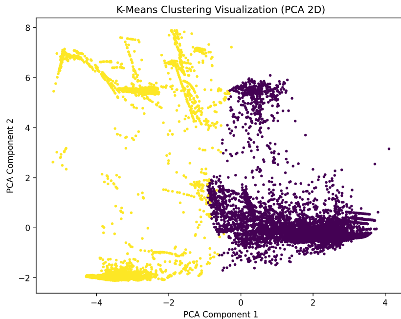
Figure 9: PCA 2D scatter plot of K-Means clusters for Dataset 1. Each point is projected onto the first two principal components of \mathbf{X}_{\text{scaled}} ; color indicates K-Means assignment in the original 41-D space.
