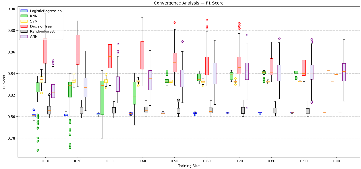
Figure 8: Convergence box plots, Weighted F1, Dataset 2.
