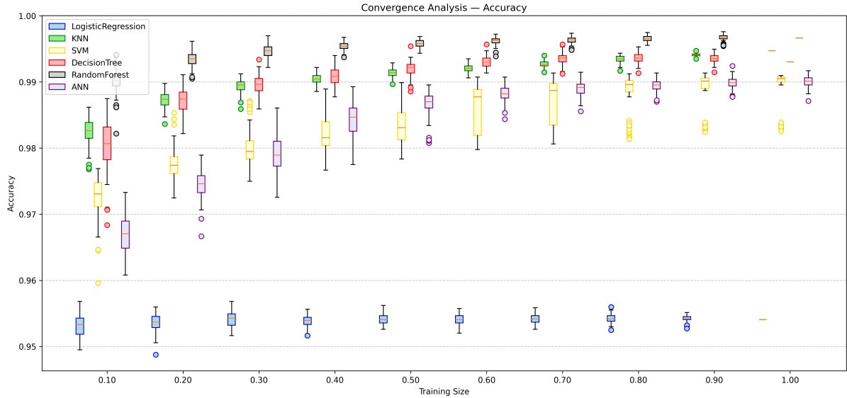
Figure 5: Convergence box plots, Accuracy, Dataset 1. Each box summarizes 100 iterations at the corresponding training fraction.
