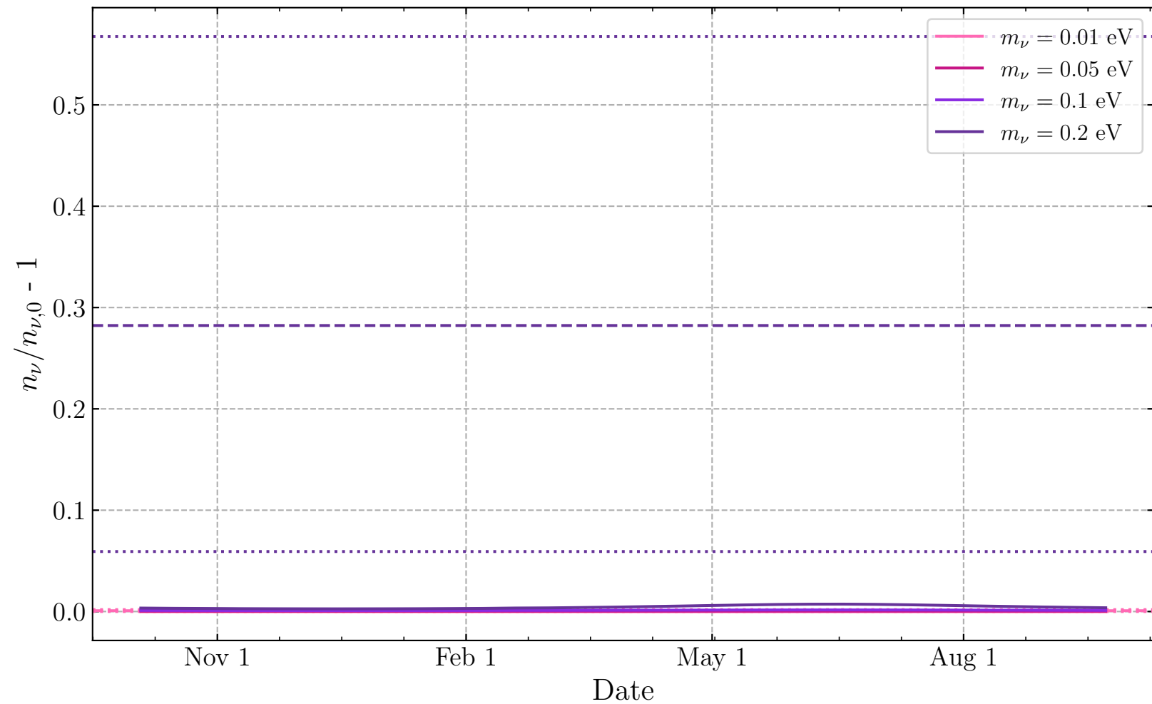
Number densities
