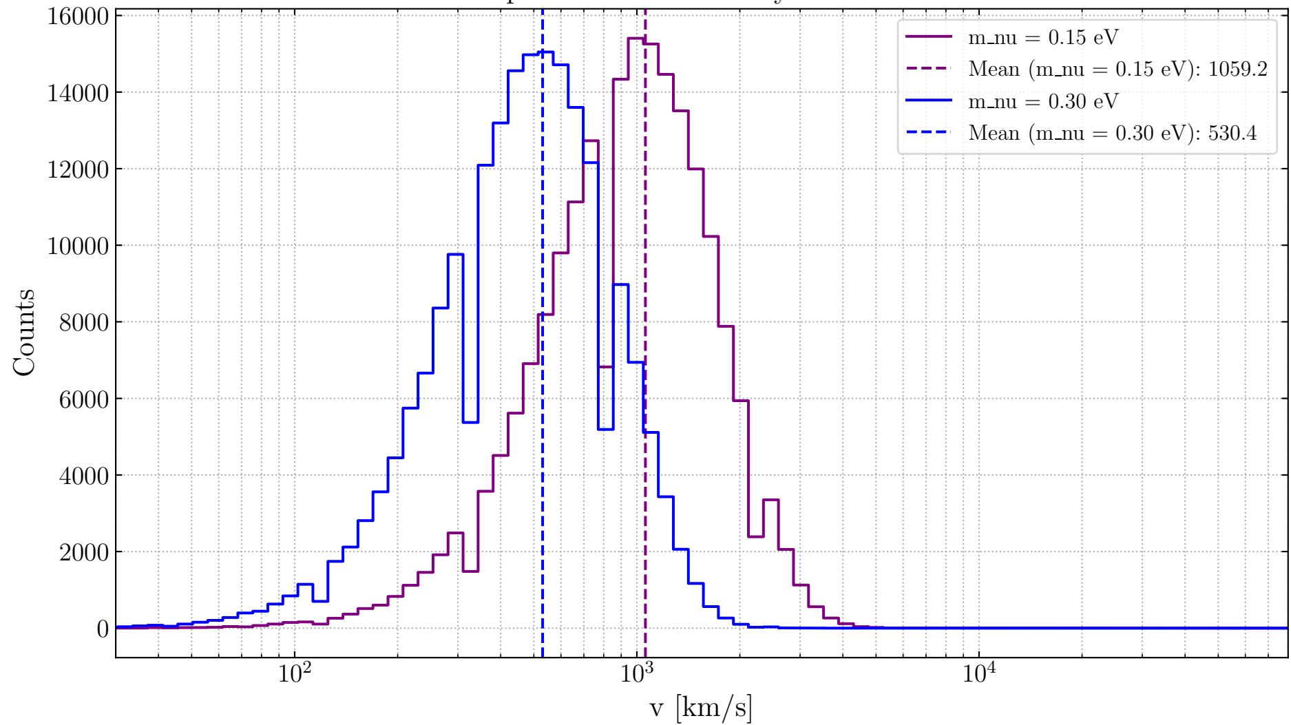
Sampled Neutrino Velocity Distribution
