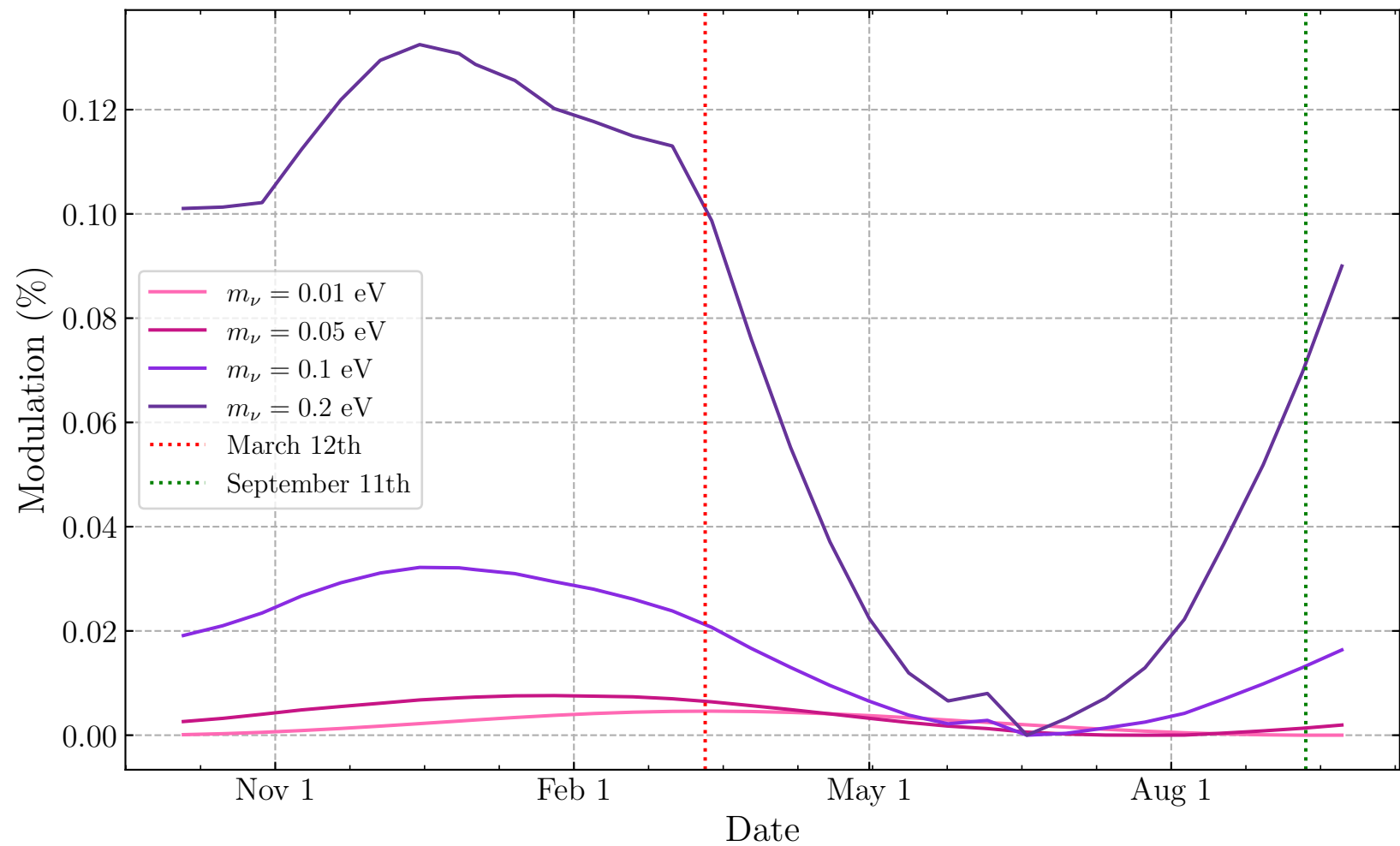
Annual modulation
