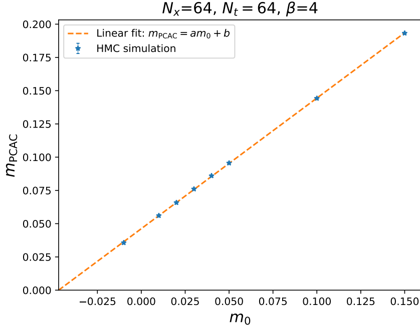
Figure 6: We fit a linear function to m_{\text{PCAC}}(m_0) in order to determine the critical mass at \beta = 4 with c_{\text{sw}} = 1 . Our fit yields m_c = -0.0471(1) .
