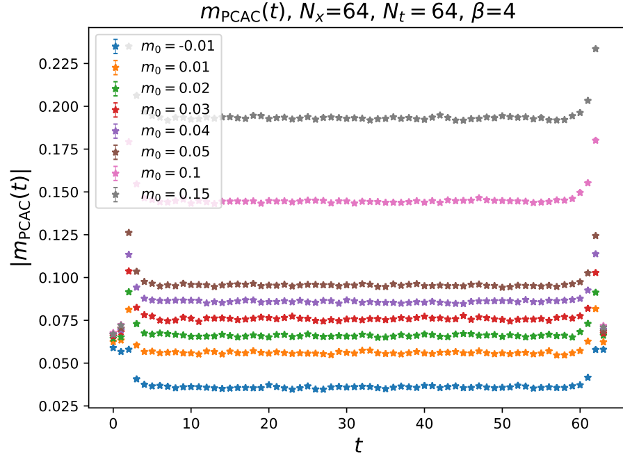
Figure 5: PCAC mass measured with eq. (26) for different values of the bare mass. To fit the plateau we consider the range t \in [10, 25] .
