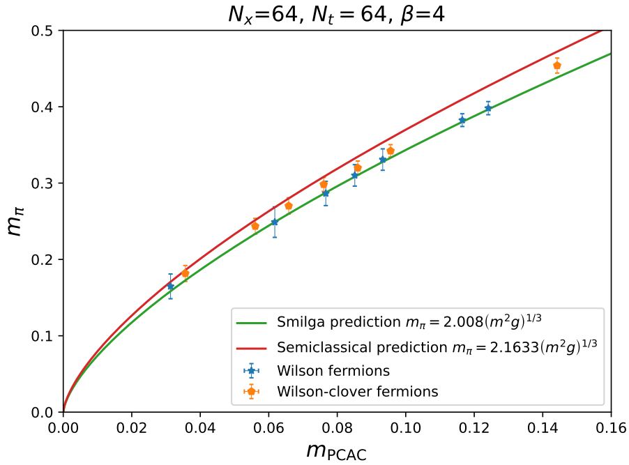
Figure 7: Behavior of m_\pi vs. m_{\text{PCAC}} for fermions with and without clover improvement. The exact numbers are displayed in Tables 1 and 2. The gauge couplings is related to \beta = 1/g^2 .
