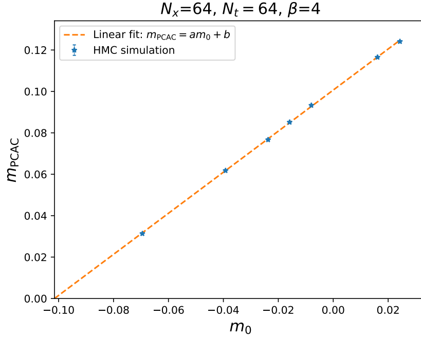
Figure 4: We fit a linear function to m_{\text{PCAC}}(m_0) in order to determine the critical mass at \beta = 4 . Our fit yields m_c = -0.1022(3) .
