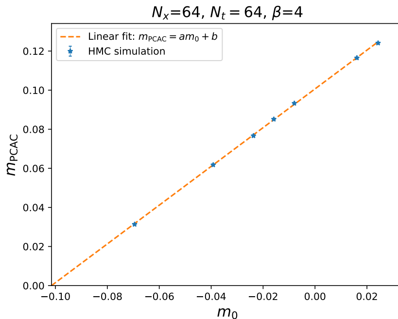
Figure 4: We fit a linear function to m_{\text{PCAC}}(m_0) in order to determine the critical mass at \beta = 4 . Our fit yields m_c = -0.1015(4) .
