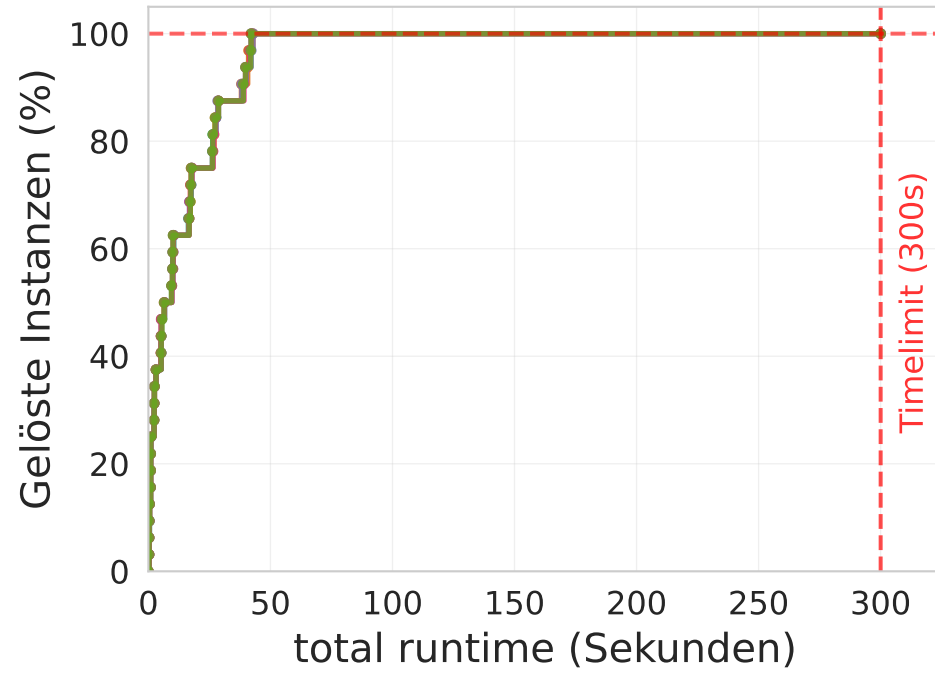
Delaunay-Flips
