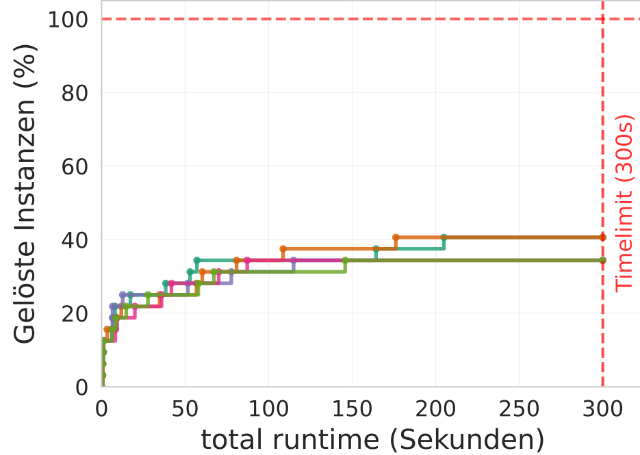
Delaunay-Flips
