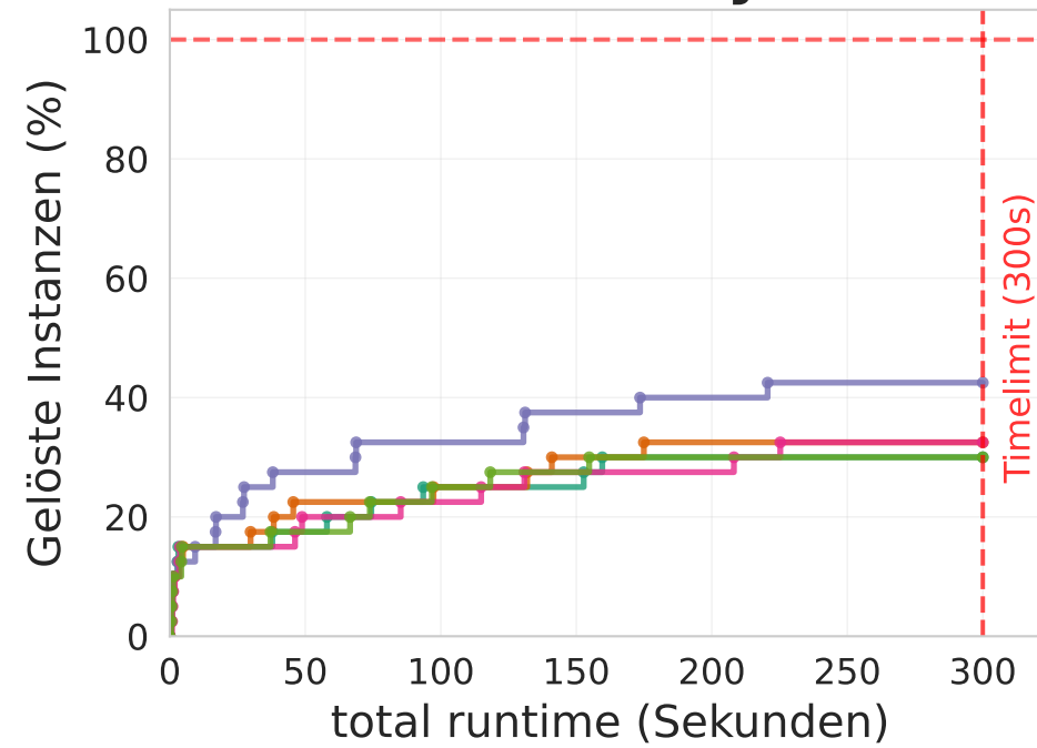
Random
