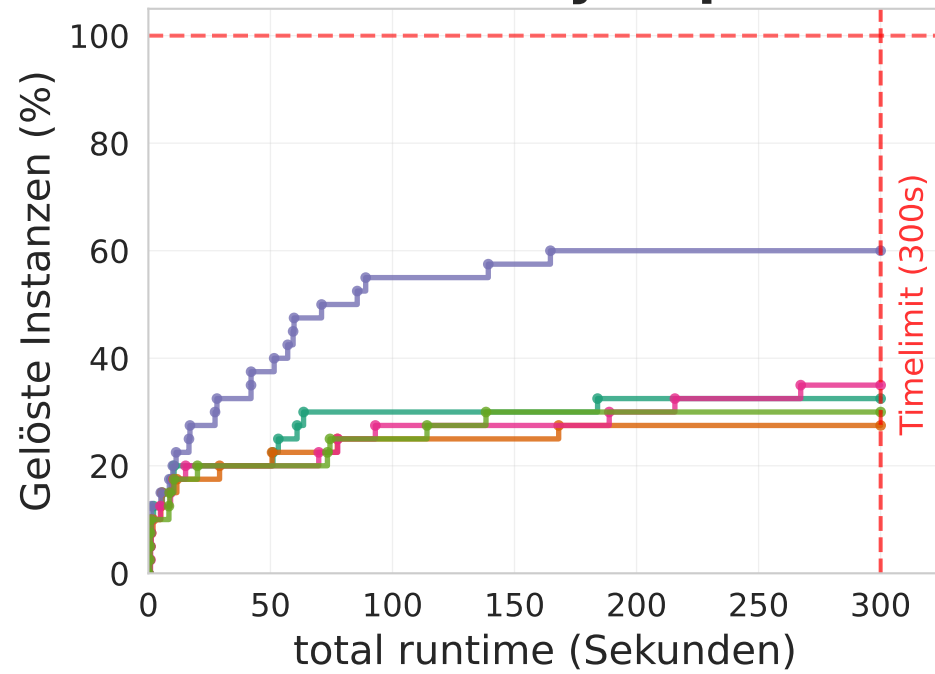
Iterative
