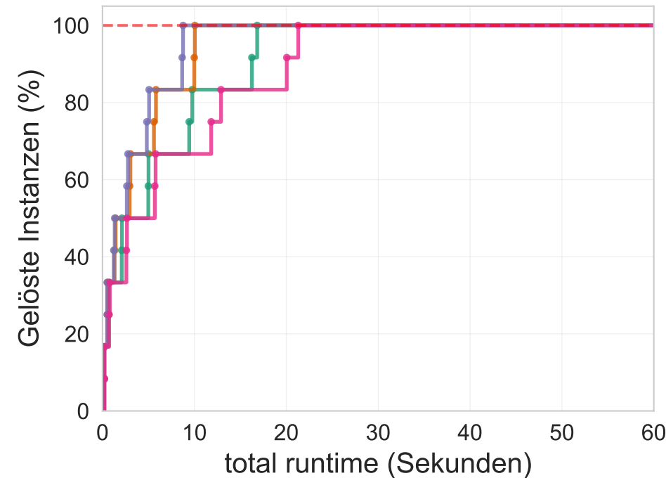
Random
