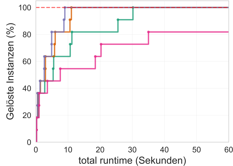
Random
