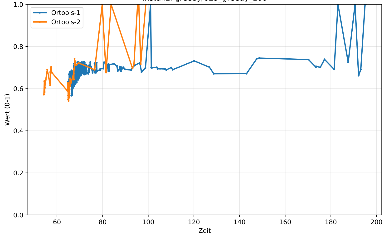
Instanz: greedy/029_greedy_100
