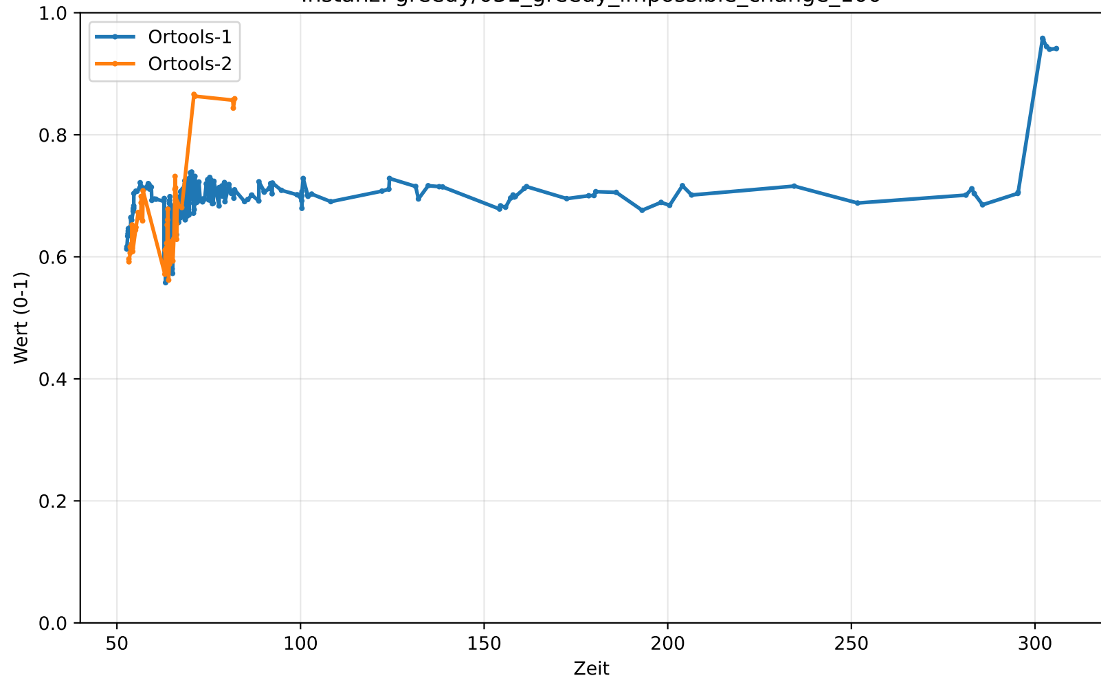
Instanz: greedy/031_greedy_impossible_change_100
